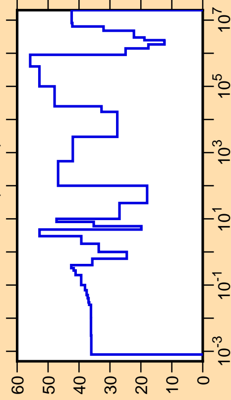
\Delta\sigma/\sigma vs. E for ^{239}\text{Th}(n,\text{tot.})
