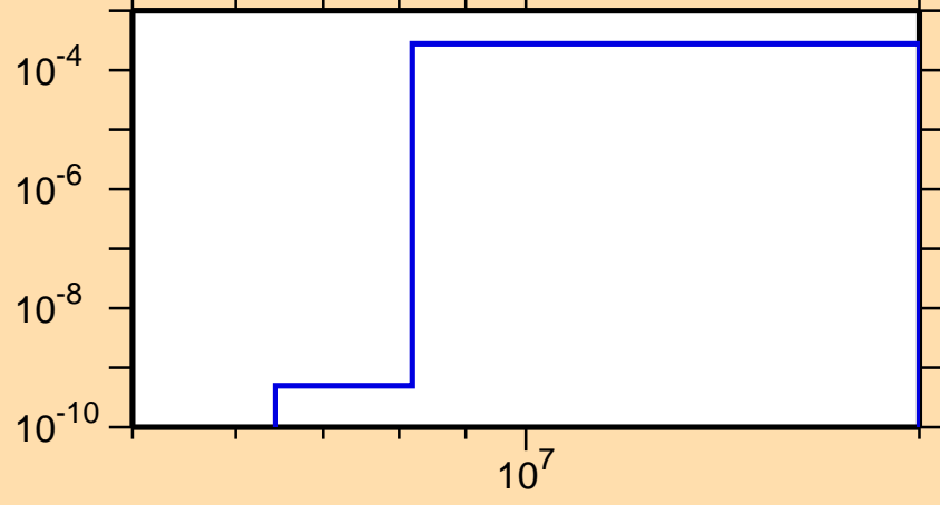
\sigma vs. E for ^{239}\text{Th}(n,p)
