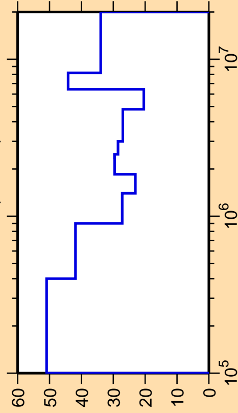
\Delta\sigma/\sigma vs. E for ^{239}\text{Th}(n,\text{inel.})
