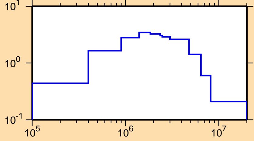
\sigma vs. E for ^{239}\text{Th}(n,\text{inel.})
