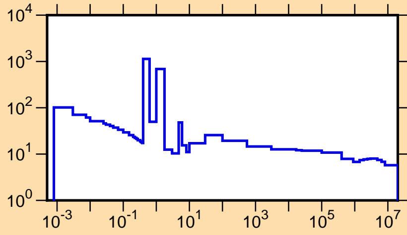
\sigma vs. E for ^{239}\text{Th}(n,\text{tot.})
