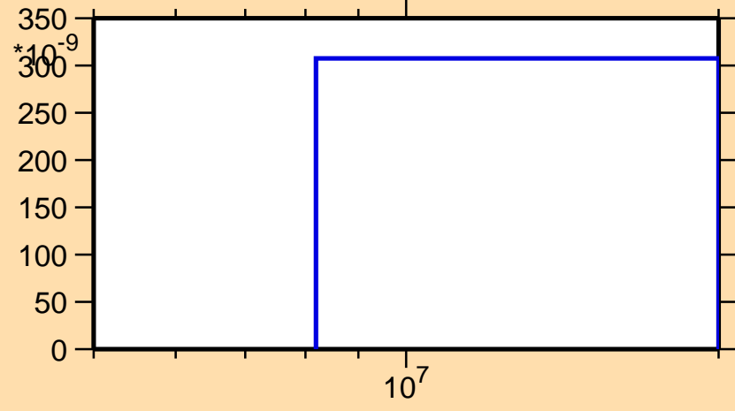
\sigma vs. E for ^{150}\text{Tm}(n,nd)
