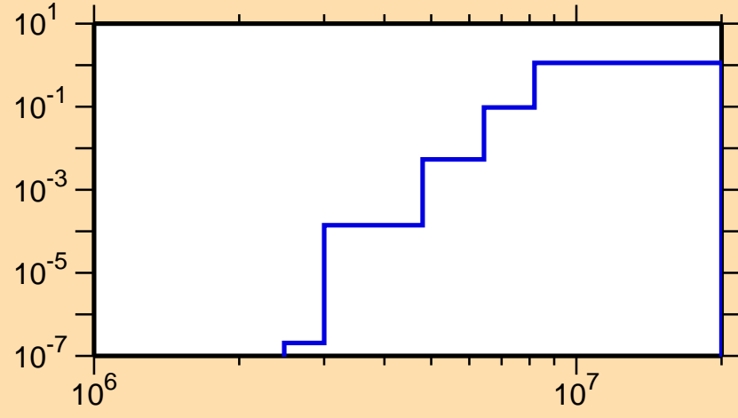
\sigma vs. E for ^{151}\text{Tm}(n,np)
