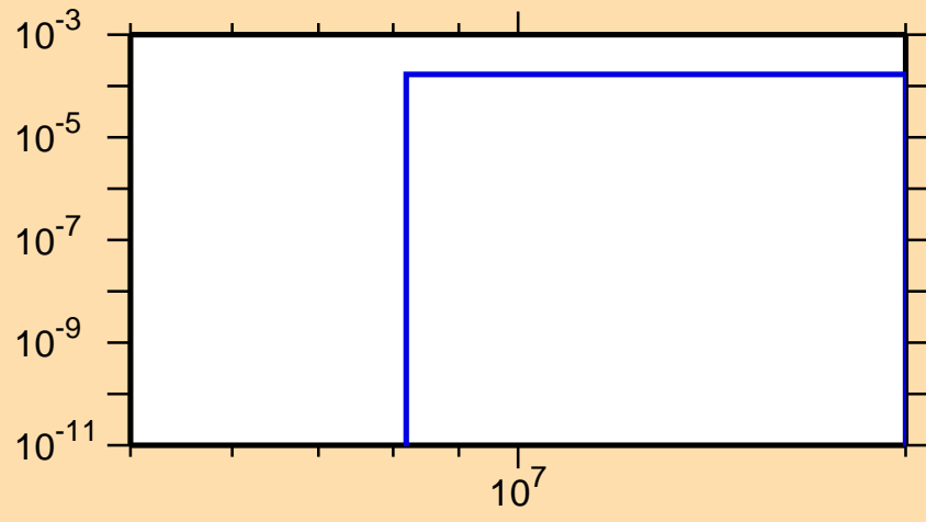
\sigma vs. E for ^{151}\text{Tm}(n,t)
