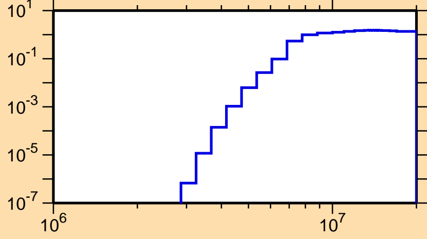
\sigma vs. E for ^{152}\text{Tm}(n,np)
