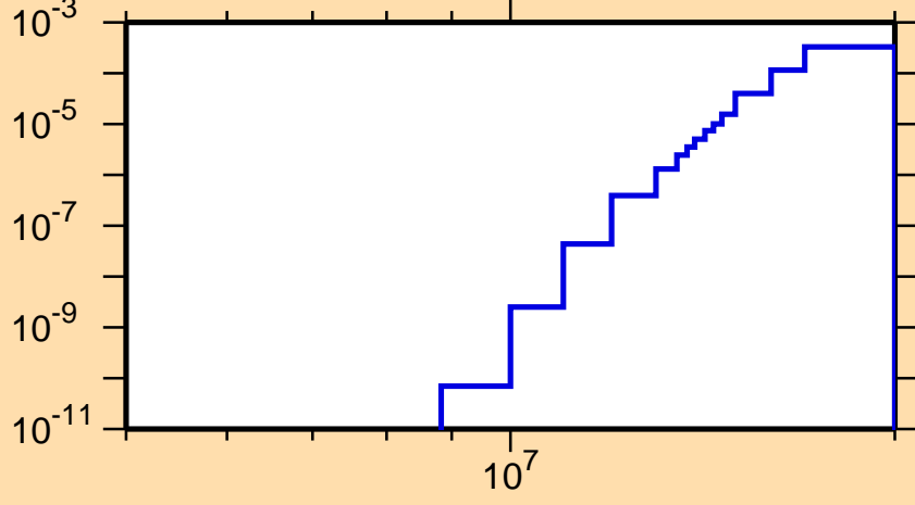
\sigma vs. E for ^{152}\text{Tm}(n,\text{pd})
