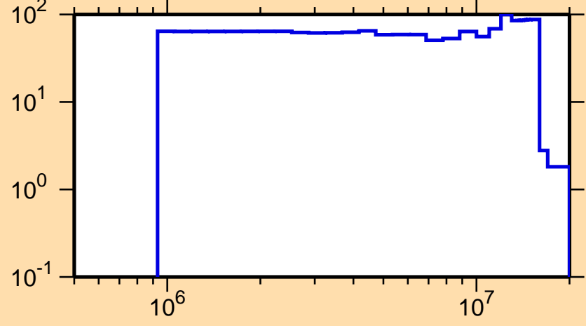
\Delta\sigma/\sigma vs. E for ^{152}\text{Tm}(n,n_1)
