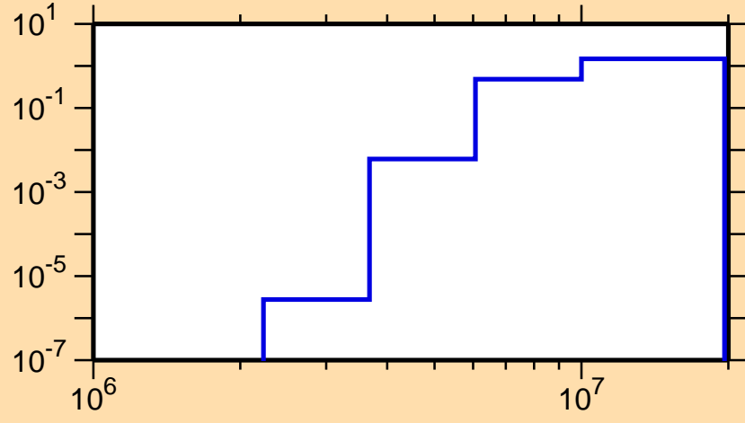
\sigma vs. E for ^{152}\text{Tm}(n,np)
