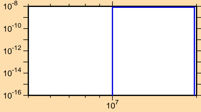
\sigma vs. E for ^{152}\text{Tm} (mt 34)
