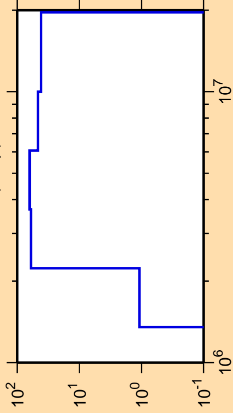
\Delta\sigma/\sigma vs. E for ^{152}\text{Tm}(n,np)
