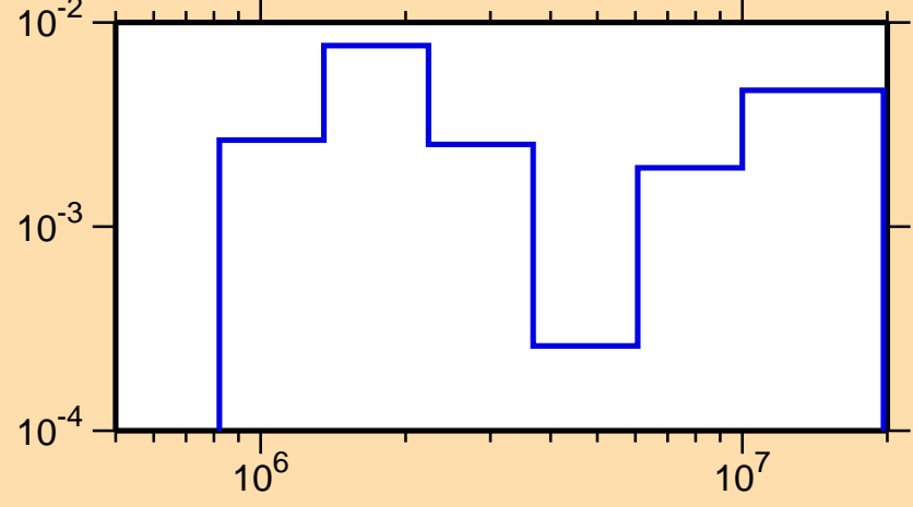
\sigma vs. E for ^{152}\text{Tm}(n,n\text{cont.})
