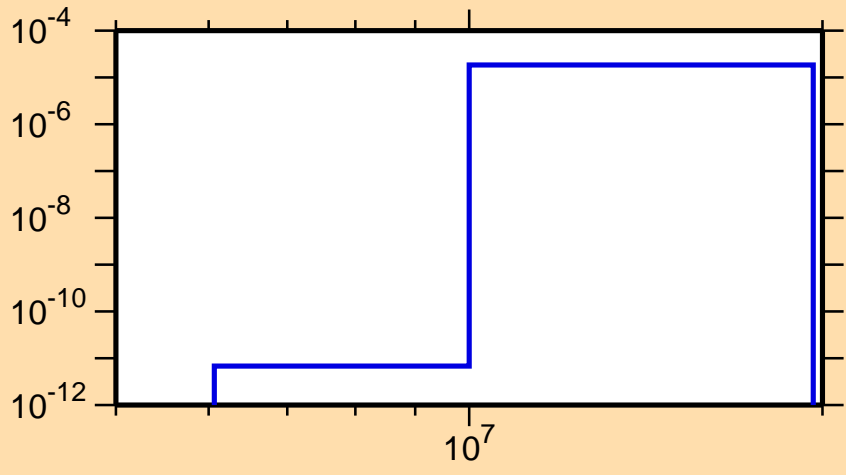
\sigma vs. E for ^{152}\text{Tm}(n,\text{pd})
