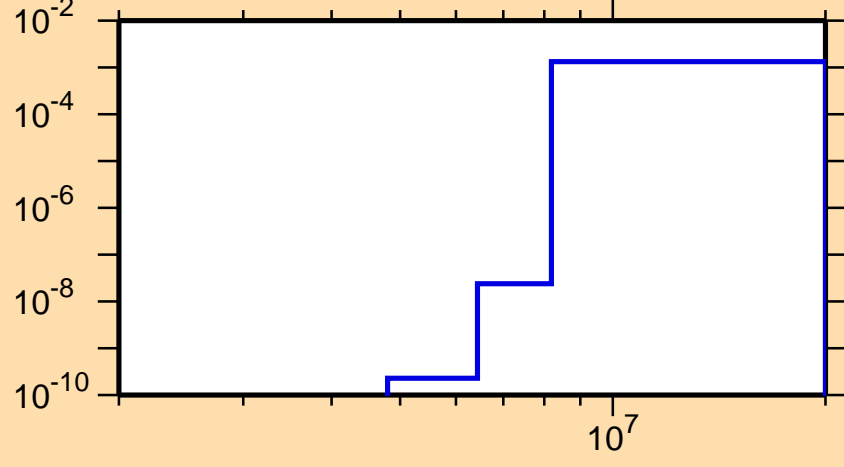
\sigma vs. E for ^{152}\text{Tm}(n,t)
