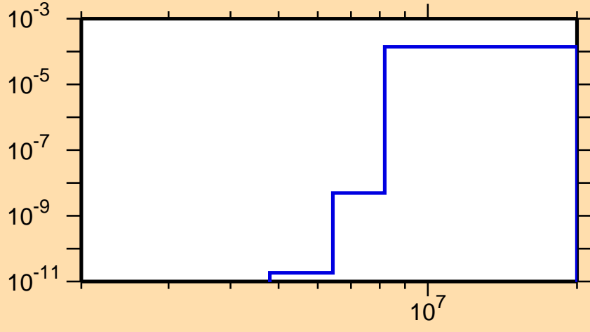
\sigma vs. E for ^{152}\text{Tm}(n,\text{He3})
