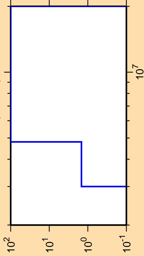
\Delta\sigma/\sigma vs. E for ^{152}\text{Tm}(n,\text{He3})
