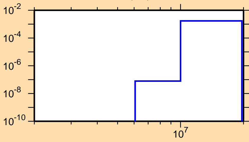
\sigma vs. E for ^{152}\text{Tm}(n,t)
