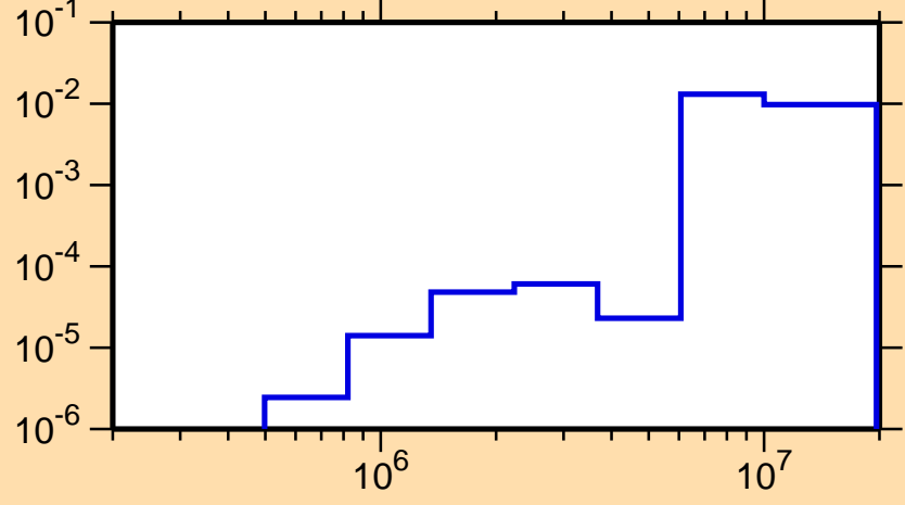
\sigma vs. E for ^{152}\text{Tm}(n,\text{inel.})
