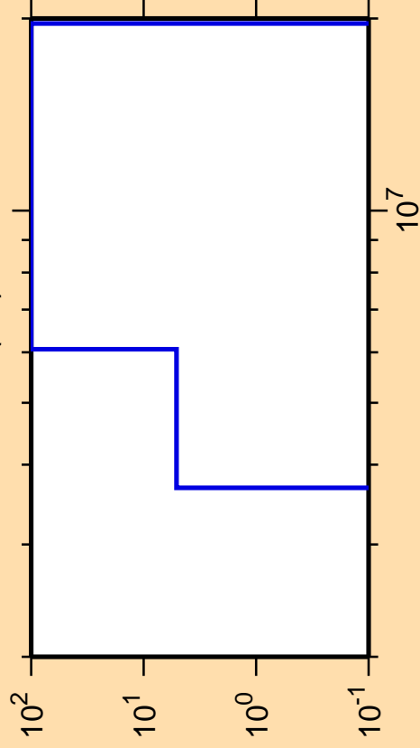
\Delta\sigma/\sigma vs. E for ^{152}\text{Tm}(n,t)
