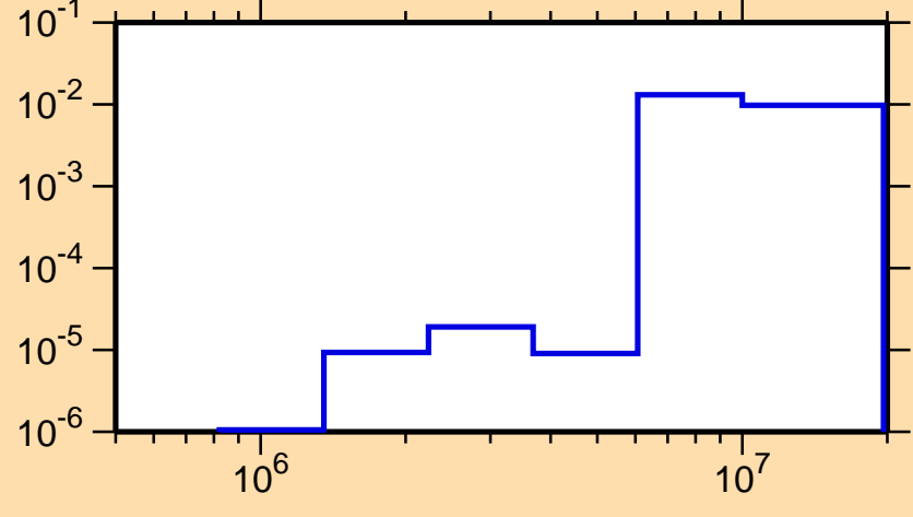
\sigma vs. E for ^{152}\text{Tm}(n,n\text{cont.})
