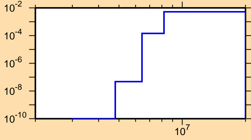
\sigma vs. E for ^{152}\text{Tm}(n,n\alpha)
