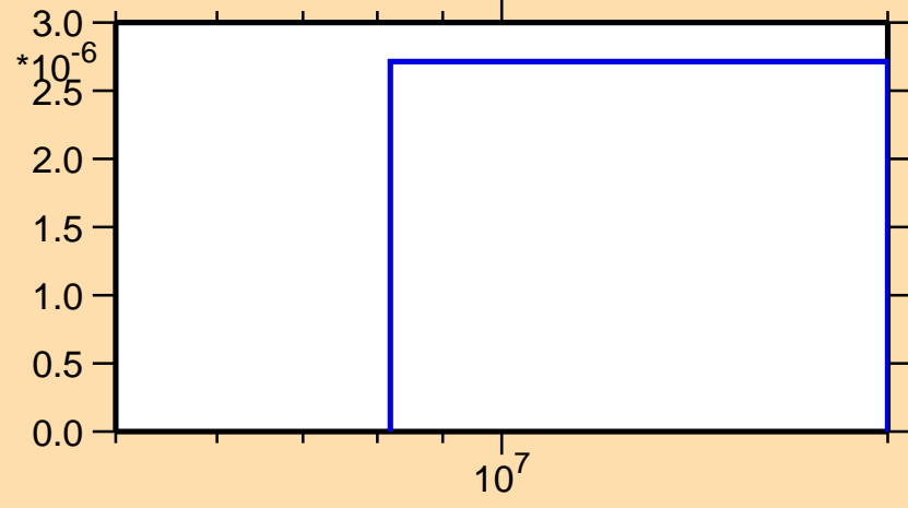
\sigma vs. E for ^{152}\text{Tm}(n,nd)
