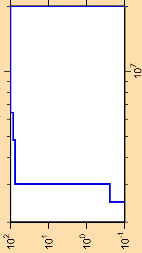
\Delta\sigma/\sigma vs. E for ^{152}\text{Tm}(n,n\alpha)
