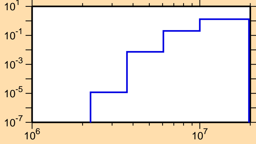
\sigma vs. E for ^{153}\text{Tm}(n,np)
