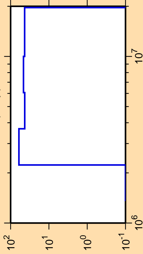
\Delta\sigma/\sigma vs. E for ^{153}\text{Tm}(n,np)
