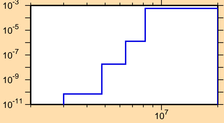
\sigma vs. E for ^{153}\text{Tm}(\text{mt117})
