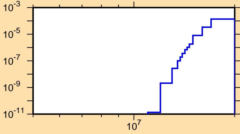
\sigma vs. E for ^{153}\text{Tm}(n,nd)
