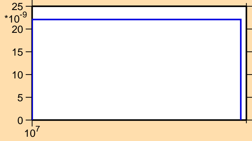
\sigma vs. E for ^{153}\text{Tm}(n,pt)
