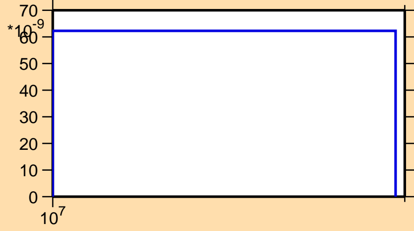
\sigma vs. E for ^{153}\text{Tm}(n,2n\alpha)
