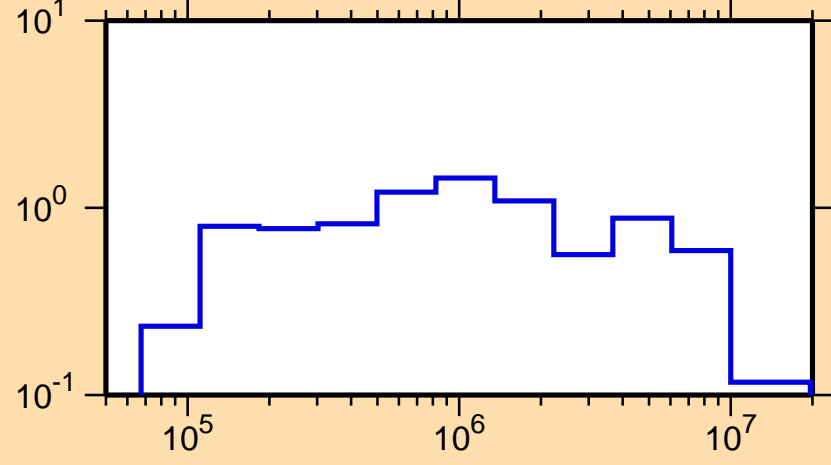
\sigma vs. E for ^{153}\text{Tm}(n,\text{inel.})
