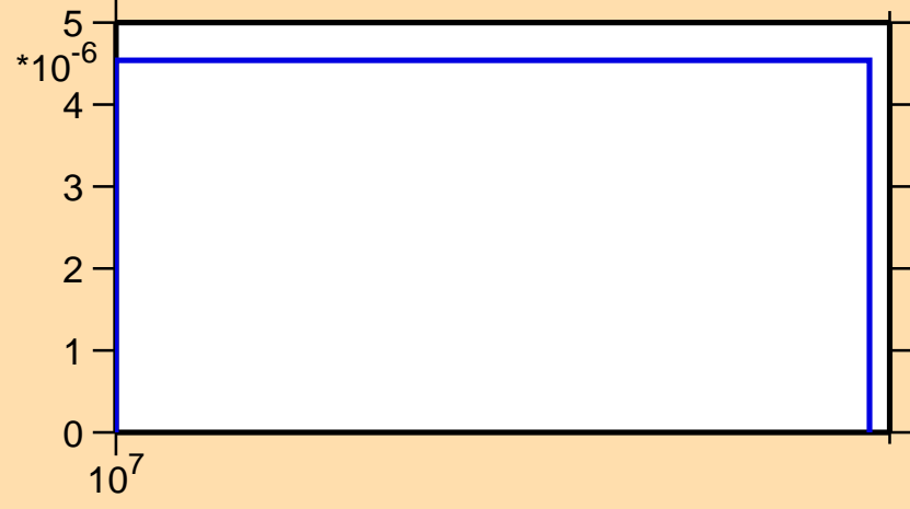
\sigma vs. E for ^{153}\text{Tm}(n,nd)
