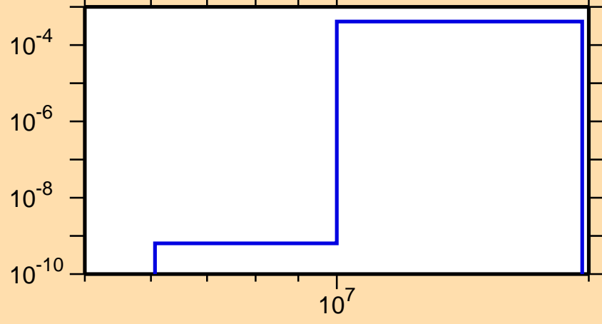
\sigma vs. E for ^{153}\text{Tm}(n,t)
