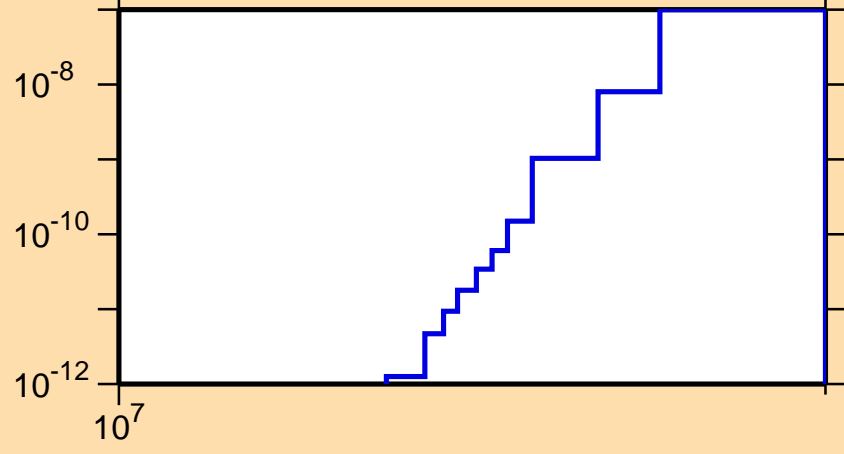
\sigma vs. E for ^{154}\text{Tm} (mt 34)
