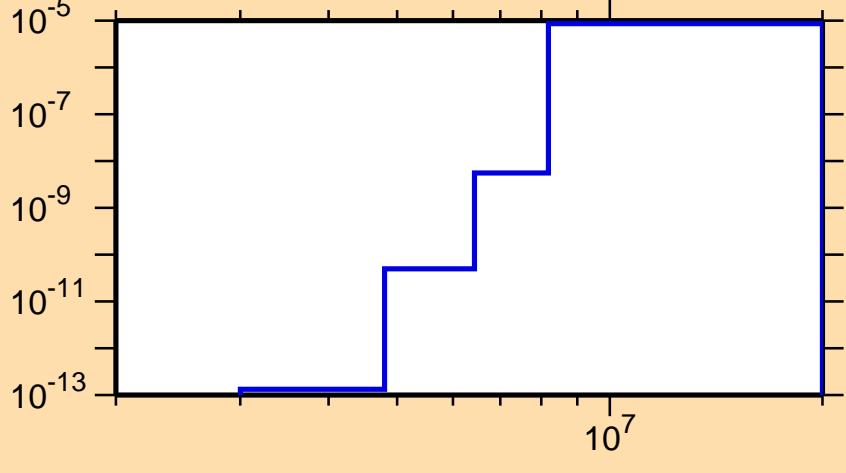
\sigma vs. E for ^{154}\text{Tm}(\text{mt117})
