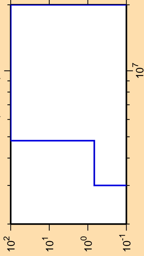
\Delta\sigma/\sigma vs. E for ^{154}\text{Tm}(\text{mt117})
