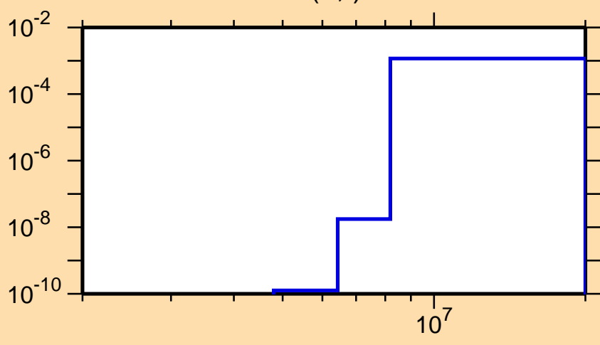
\sigma vs. E for ^{154}\text{Tm}(n,t)
