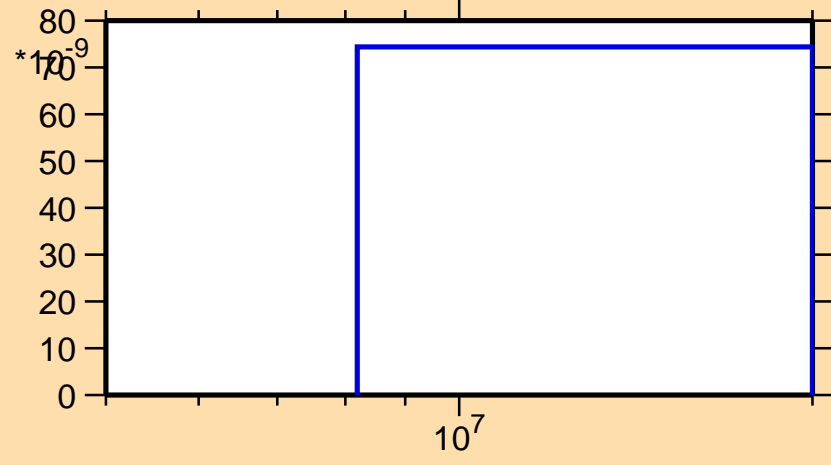
\sigma vs. E for ^{154}\text{Tm}(n,3n)
