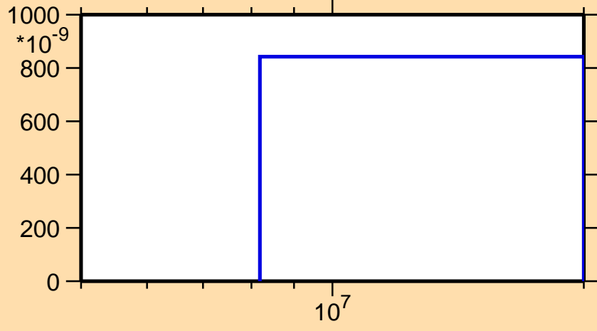
\sigma vs. E for ^{154}\text{Tm}(n,\text{pd})
