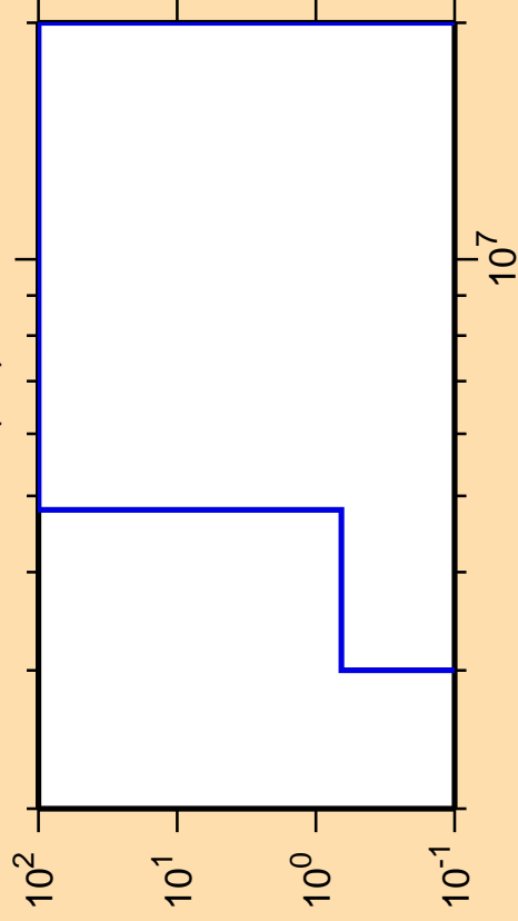
\Delta\sigma/\sigma vs. E for ^{154}\text{Tm}(n,t)
