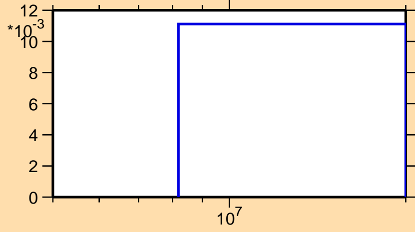
\sigma vs. E for ^{154}\text{Tm}(n,2np)
