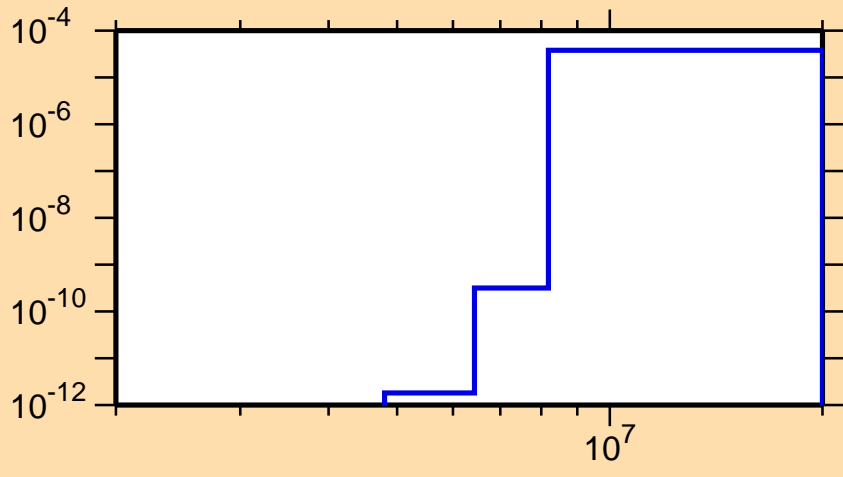
\sigma vs. E for ^{154}\text{Tm}(n,\text{He3})
