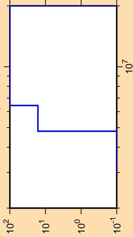
\Delta\sigma/\sigma vs. E for ^{154}\text{Tm}(n,\text{He3})
