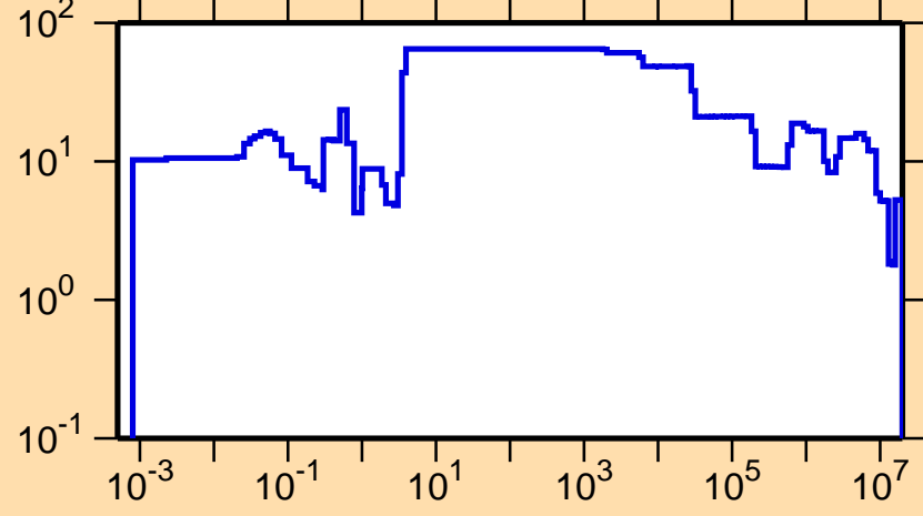
\Delta\sigma/\sigma vs. E for ^{154}\text{Tm}(n,\text{tot.})
