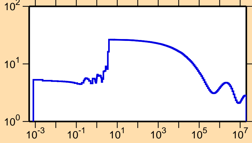
\sigma vs. E for ^{154}\text{Tm}(n,\text{el.})
