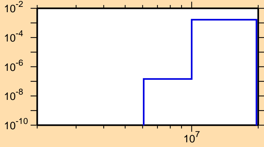
\sigma vs. E for ^{154}\text{Tm}(n,t)
