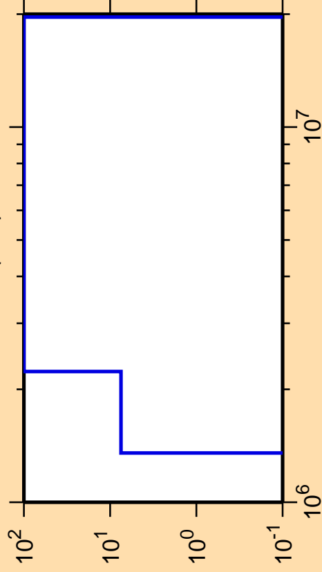
\Delta\sigma/\sigma vs. E for ^{154}\text{Tm}(n,d)
