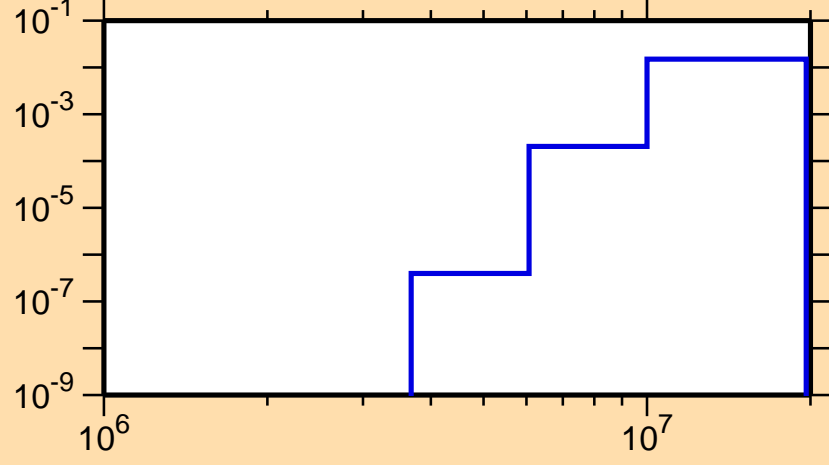
\sigma vs. E for ^{154}\text{Tm}(n,d)
