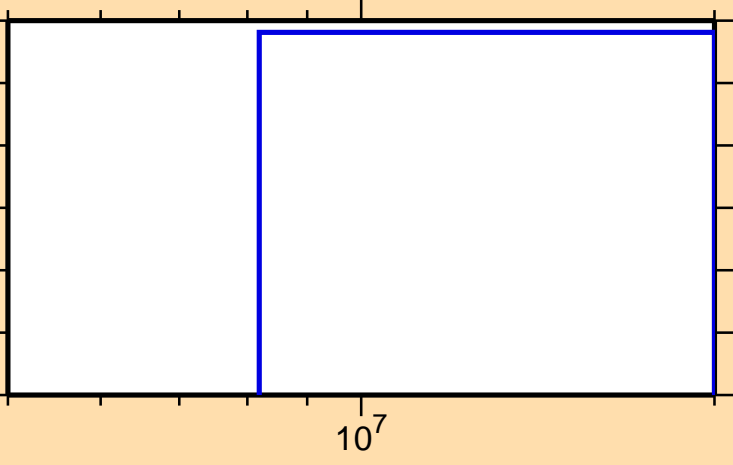
\sigma vs. E for ^{154}\text{Tm}(n,2n)
