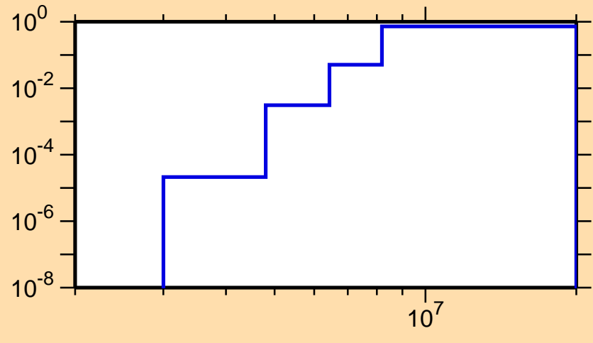
\sigma vs. E for ^{154}\text{Tm}(n,np)
