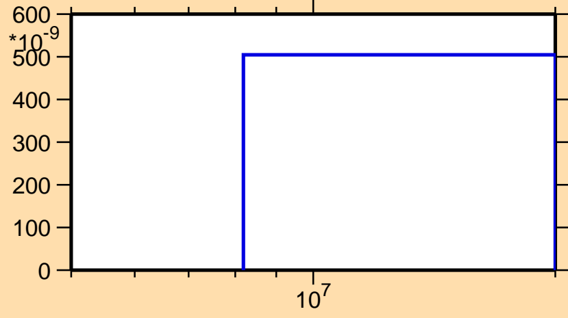
\sigma vs. E for ^{154}\text{Tm}(n,\text{pd})
