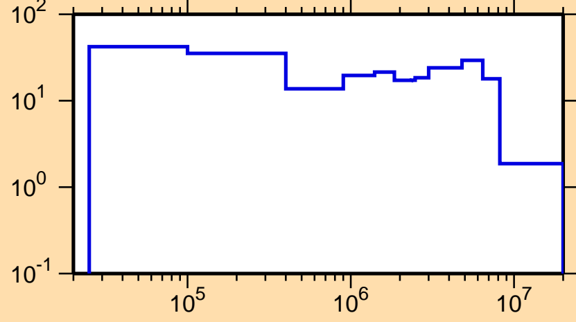
\Delta\sigma/\sigma vs. E for ^{154}\text{Tm}(n,\text{el.})
