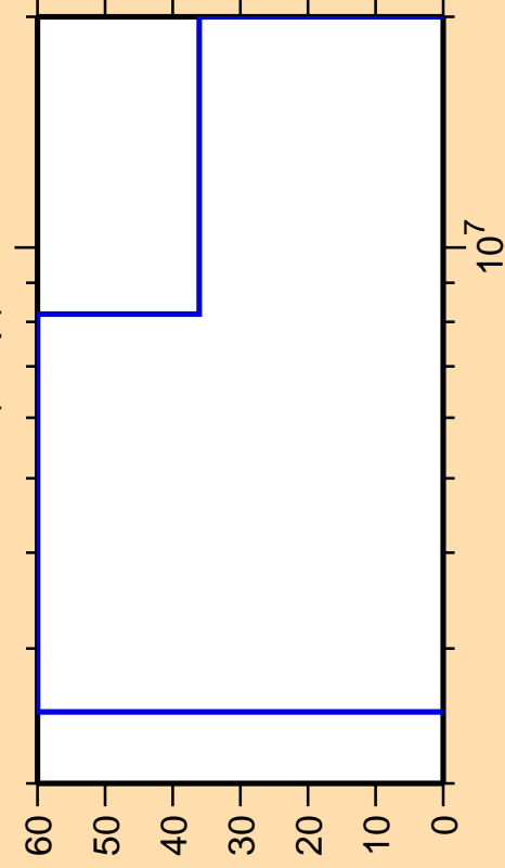
\Delta\sigma/\sigma vs. E for ^{154}\text{Tm}(n,np)
