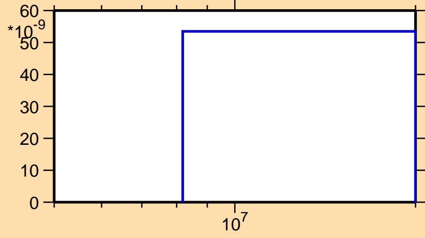
\sigma vs. E for ^{154}\text{Tm}(n,pt)
