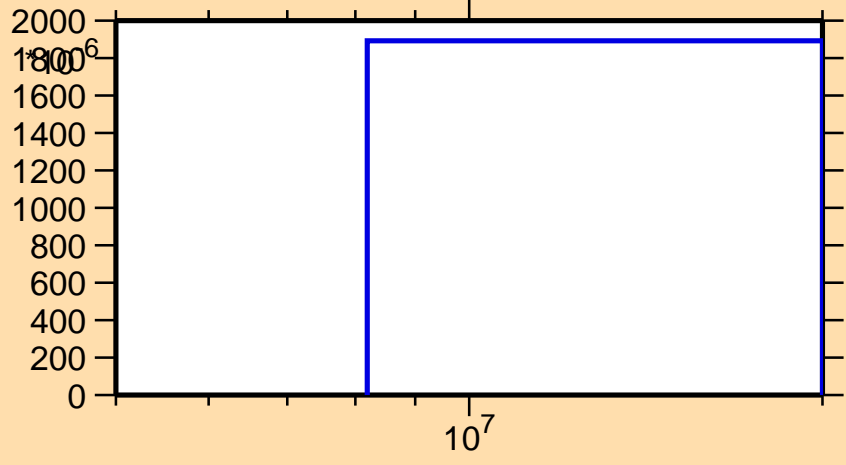
\sigma vs. E for ^{154}\text{Tm}(n,2n\alpha)
