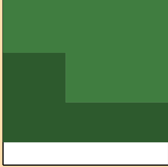
\Delta\sigma/\sigma vs. E for ^{155}\text{Tm}(n,\text{nonel.})
