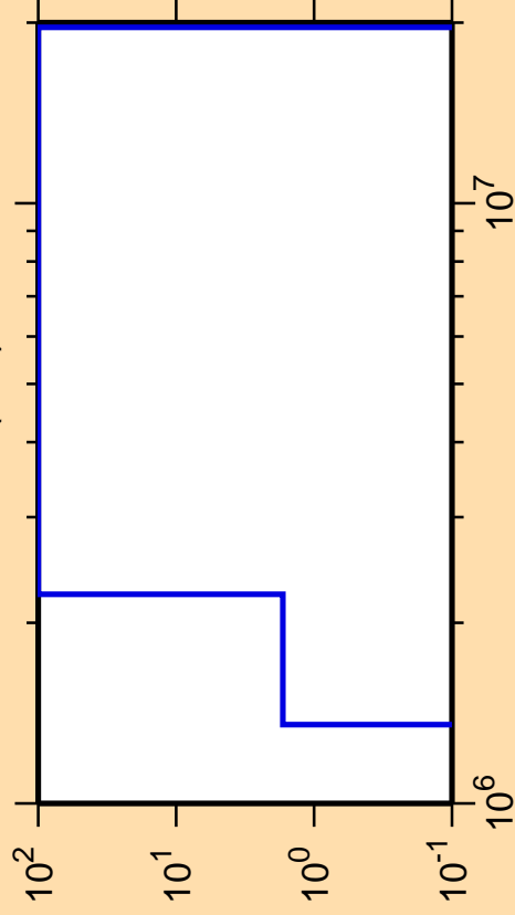
\Delta\sigma/\sigma vs. E for ^{155}\text{Tm}(n,d)
