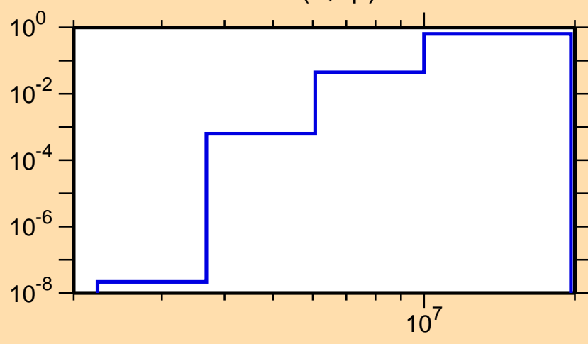
\sigma vs. E for ^{155}\text{Tm}(n,np)
