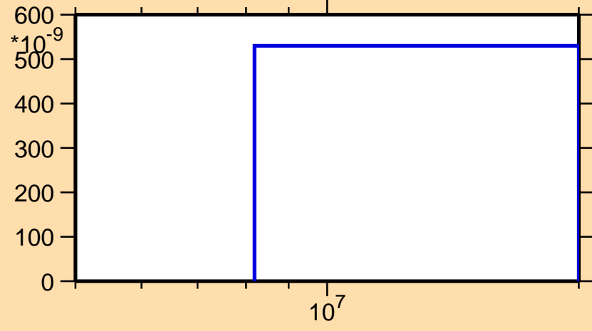
\sigma vs. E for ^{155}\text{Tm}(n,nd)
