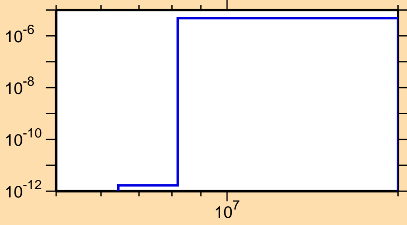
\sigma vs. E for ^{155}\text{Tm}(n,\text{He}3)
