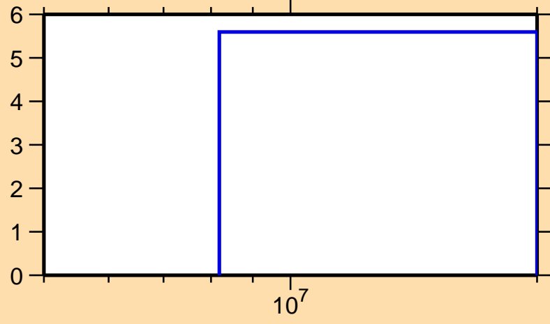
\Delta\sigma/\sigma vs. E for ^{155}\text{Tm}(n,\text{el.})
