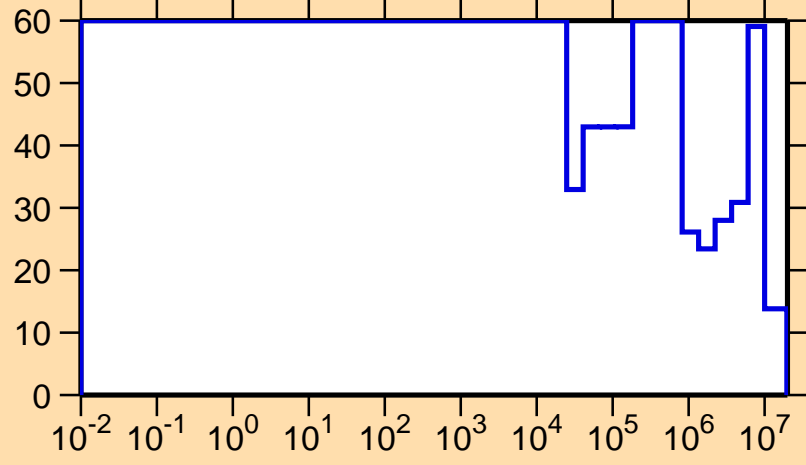
\Delta\sigma/\sigma vs. E for ^{155}\text{Tm}(n,\text{el.})
