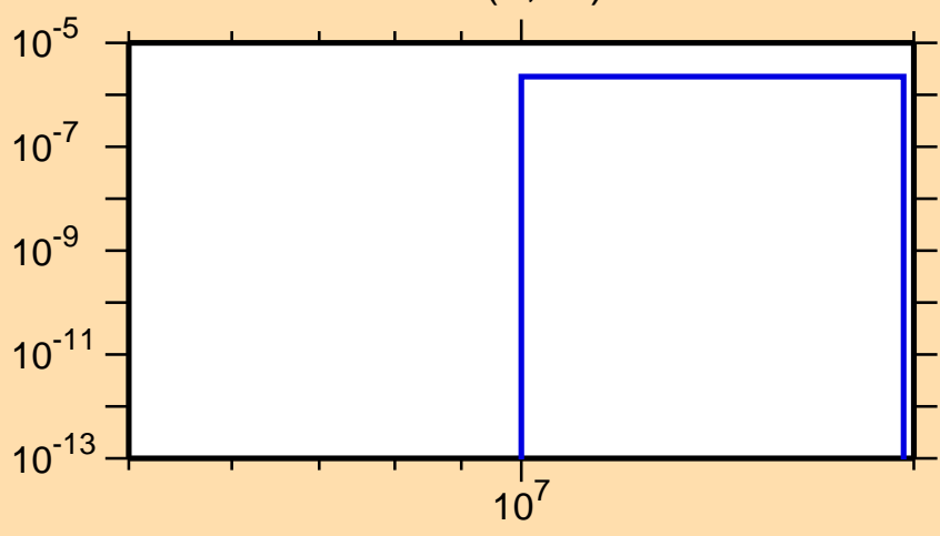
\sigma vs. E for ^{155}\text{Tm}(n,nd)
