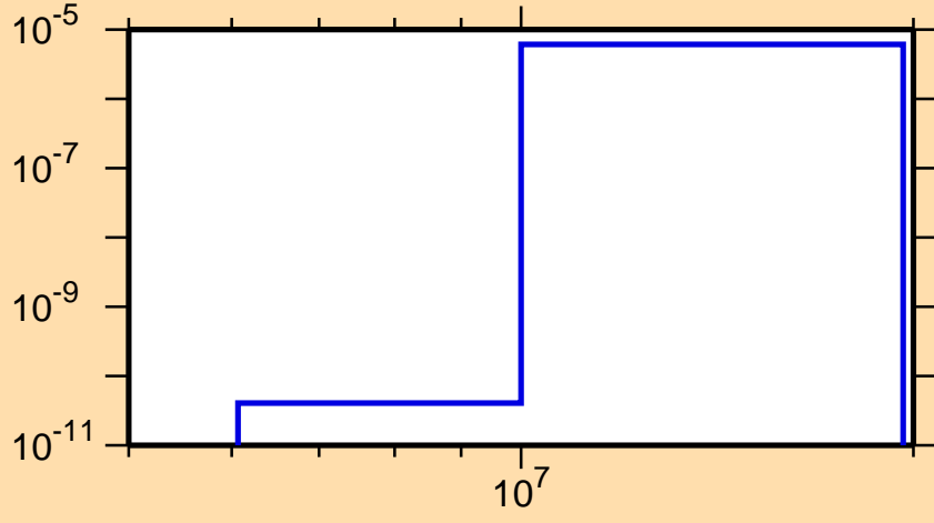
\sigma vs. E for ^{155}\text{Tm}(n,\text{He3})
