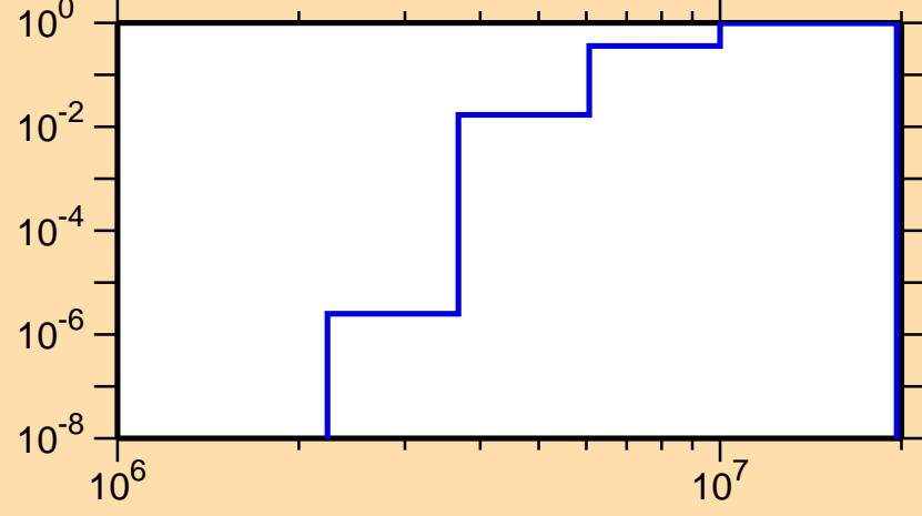
\sigma vs. E for ^{155}\text{Tm}(n,np)
