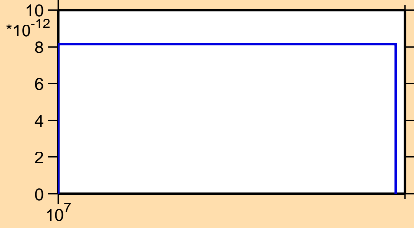
\sigma vs. E for ^{155}\text{Tm} (mt 34)
