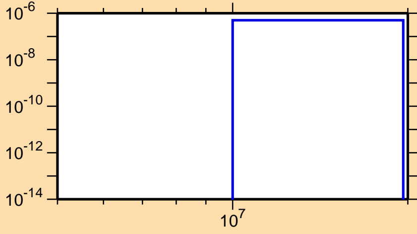
\sigma vs. E for ^{155}\text{Tm}(n,\text{pd})
