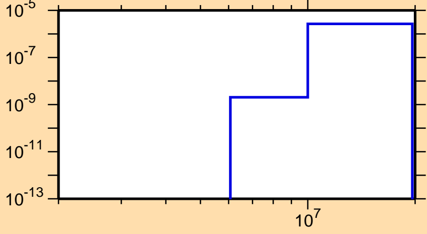
\sigma vs. E for ^{155}\text{Tm}(\text{mt117})
