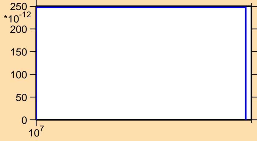
\sigma vs. E for ^{155}\text{Tm}(n,pt)
