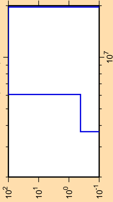
\Delta\sigma/\sigma vs. E for ^{155}\text{Tm}(\text{mt117})
