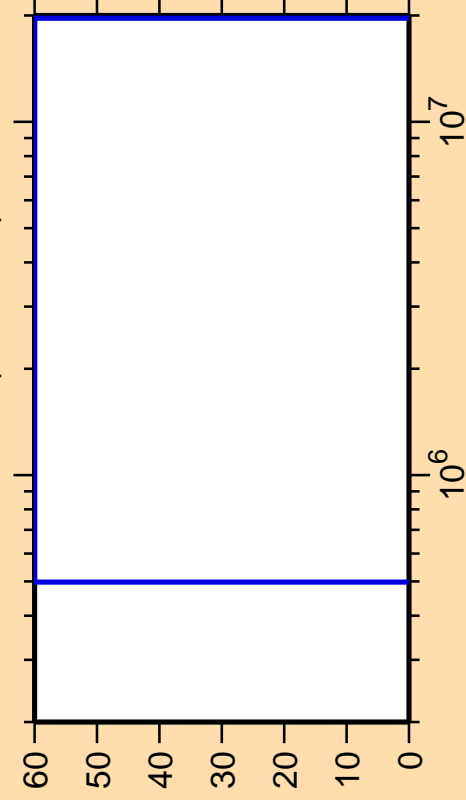
\Delta\sigma/\sigma vs. E for ^{155}\text{Tm}(n,n\text{cont.})
