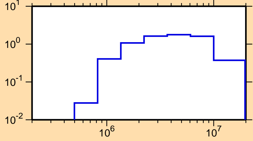
\sigma vs. E for ^{155}\text{Tm}(n,n\text{cont.})
