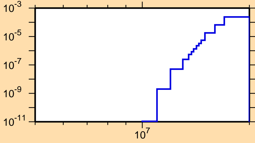
\sigma vs. E for ^{156}\text{Tm}(n,nd)
