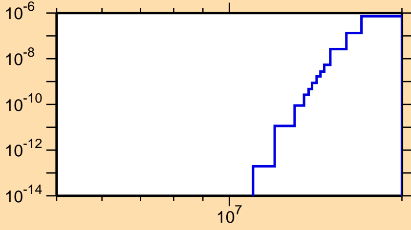
\sigma vs. E for ^{156}\text{Tm}(n,\text{pd})
