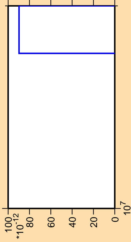
\Delta\sigma/\sigma vs. E for ^{156}\text{Tm} (mt 42)
