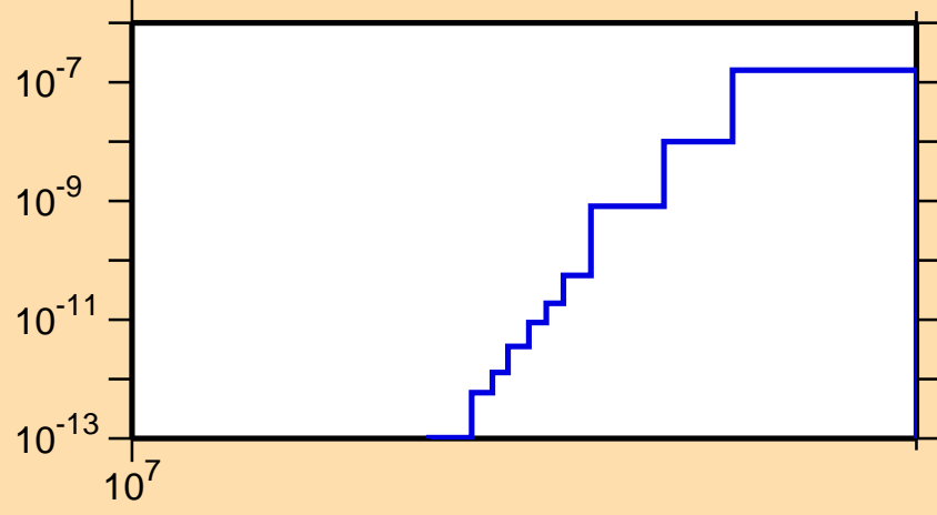
\sigma vs. E for ^{156}\text{Tm}(n,pt)
