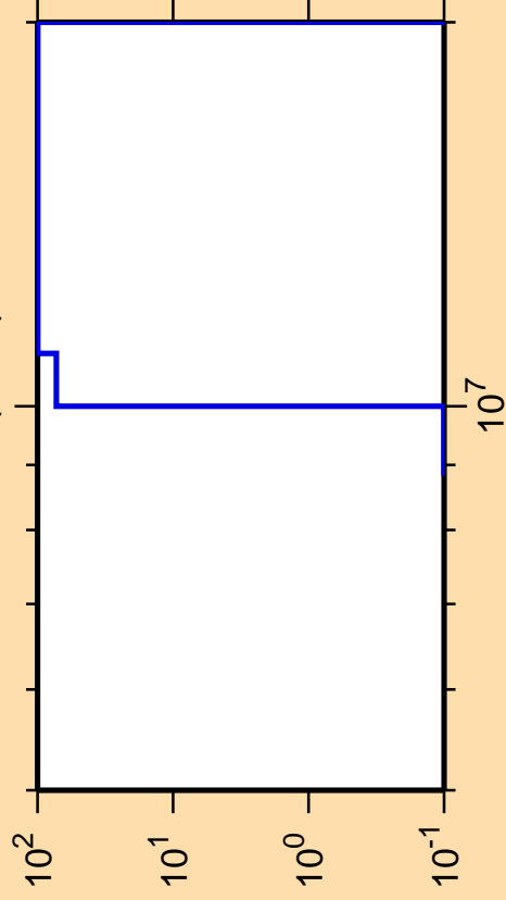
\Delta\sigma/\sigma vs. E for ^{156}\text{Tm}(n,nd)
