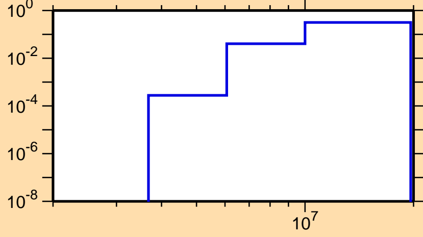
\sigma vs. E for ^{156}\text{Tm}(n,np)
