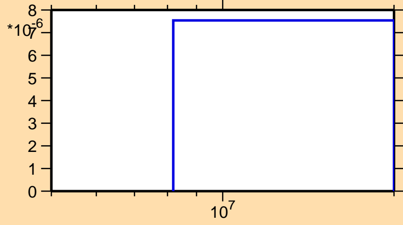
\sigma vs. E for ^{156}\text{Tm}(n,\text{nd})
