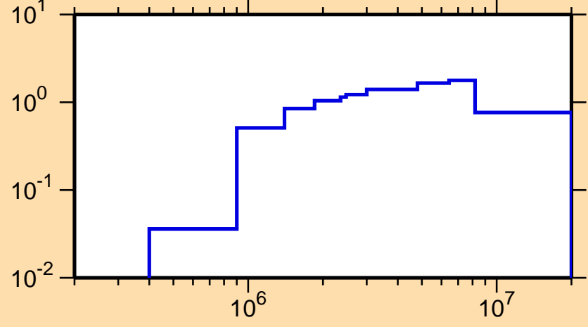
\sigma vs. E for ^{156}\text{Tm}(n,n\text{cont.})
