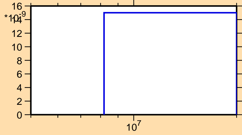
\sigma vs. E for ^{156}\text{Tm}(n,\text{pd})
