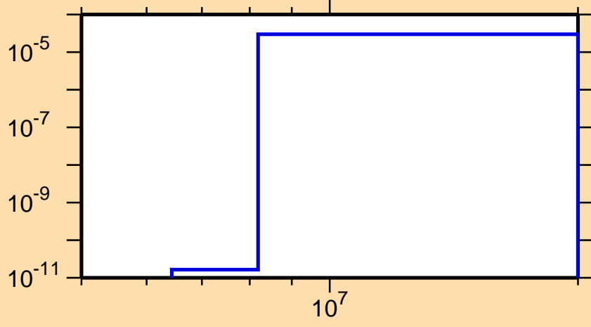
\sigma vs. E for ^{156}\text{Tm} (mt 45)
