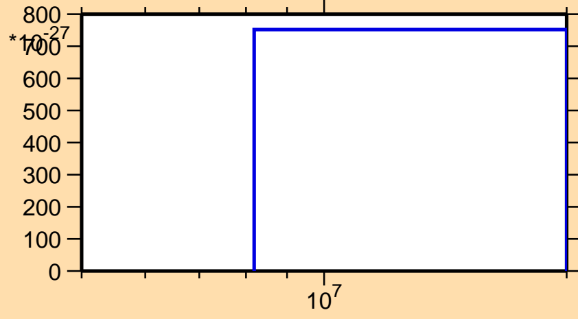
\sigma vs. E for ^{156}\text{Tm} (mt 42)
