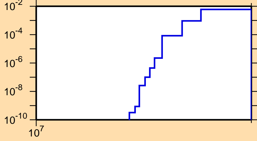
\sigma vs. E for ^{157}\text{Tm}(n,2np)
