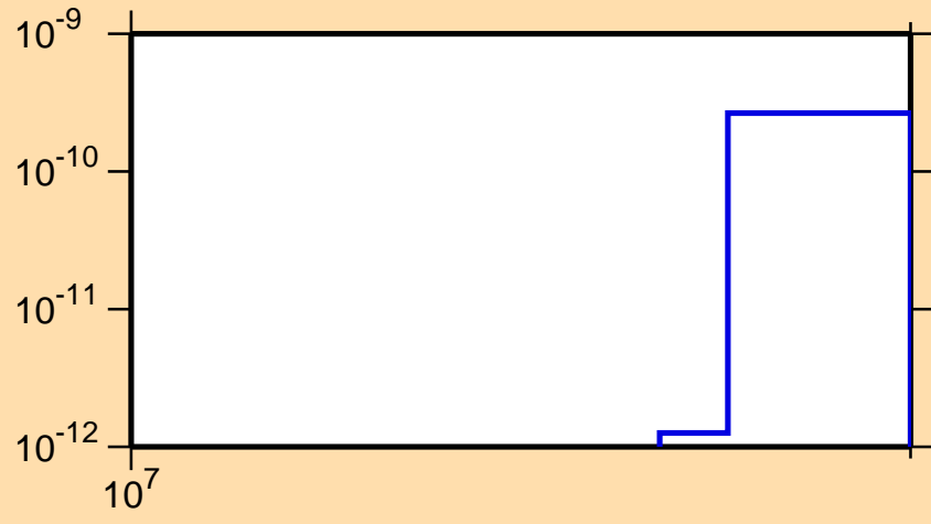
\sigma vs. E for ^{157}\text{Tm}(n,pt)
