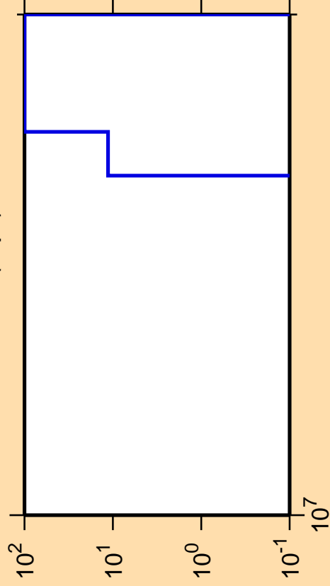
\Delta\sigma/\sigma vs. E for ^{157}\text{Tm}(n,pt)
