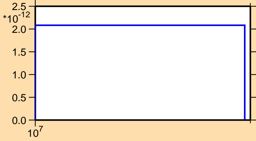
\sigma vs. E for ^{157}\text{Tm}(n,pt)
