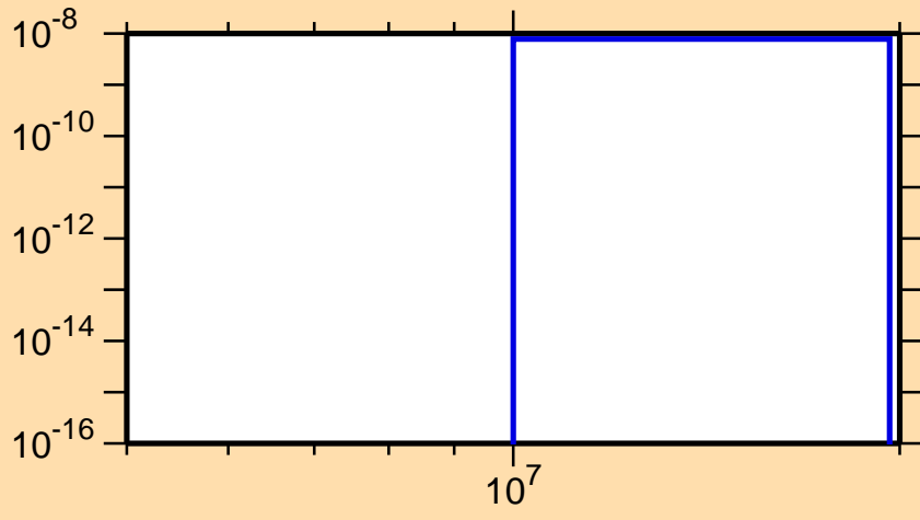
\sigma vs. E for ^{157}\text{Tm}(n,\text{pd})
