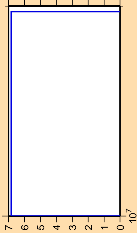
\Delta\sigma/\sigma vs. E for ^{157}\text{Tm}(n,3n\alpha)
