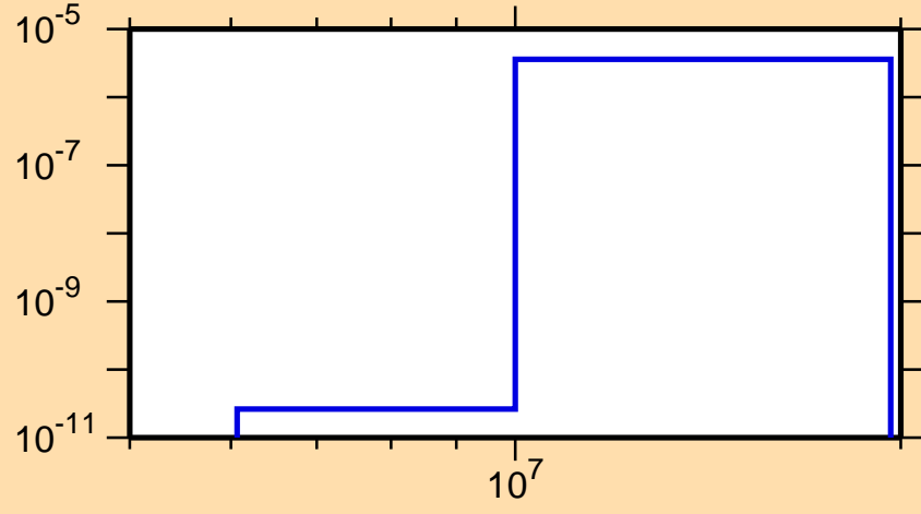
\sigma vs. E for ^{157}\text{Tm} (mt 45)
