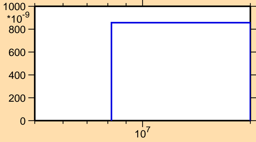
\sigma vs. E for ^{157}\text{Tm}(n,2n\alpha)
