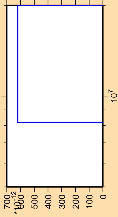
\Delta\sigma/\sigma vs. E for ^{157}\text{Tm} (mt 42)
