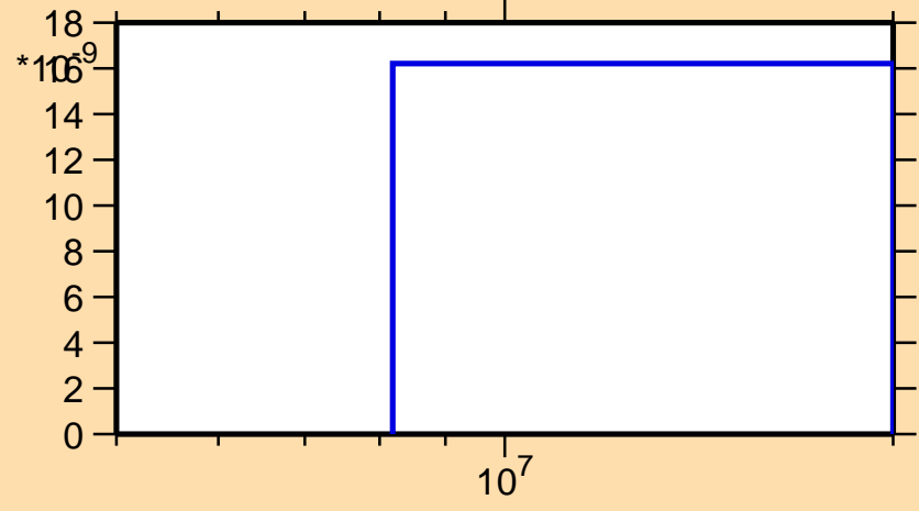
\sigma vs. E for ^{157}\text{Tm}(\text{mt117})
