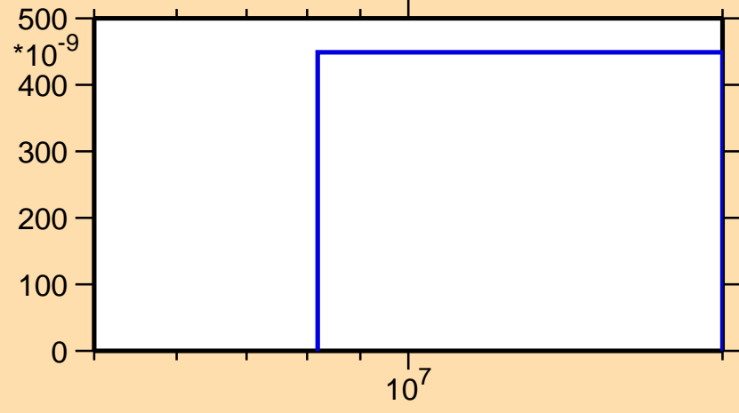
\sigma vs. E for ^{157}\text{Tm}(n,\text{nd})
