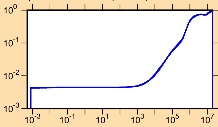
\mu vs. E for ^{158}\text{Tm}(\text{mt251})
