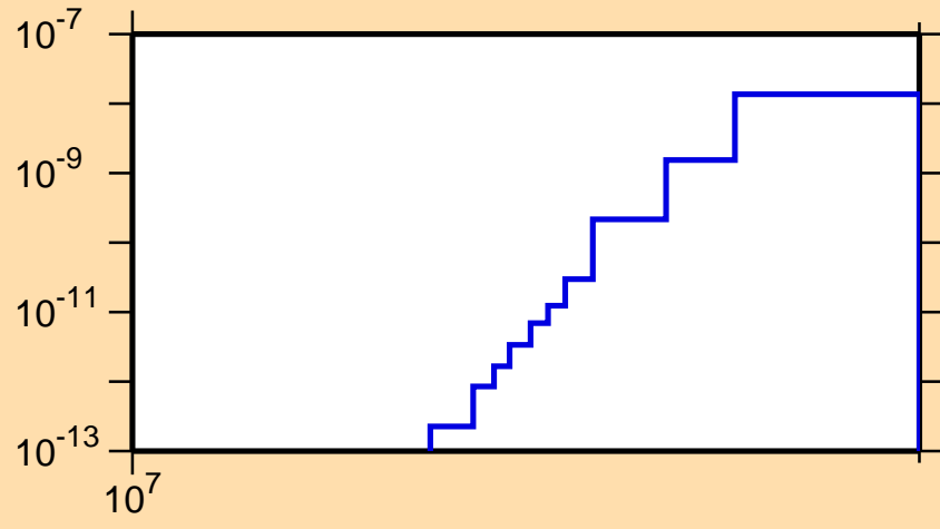
\sigma vs. E for ^{158}\text{Tm}(n,pd)
