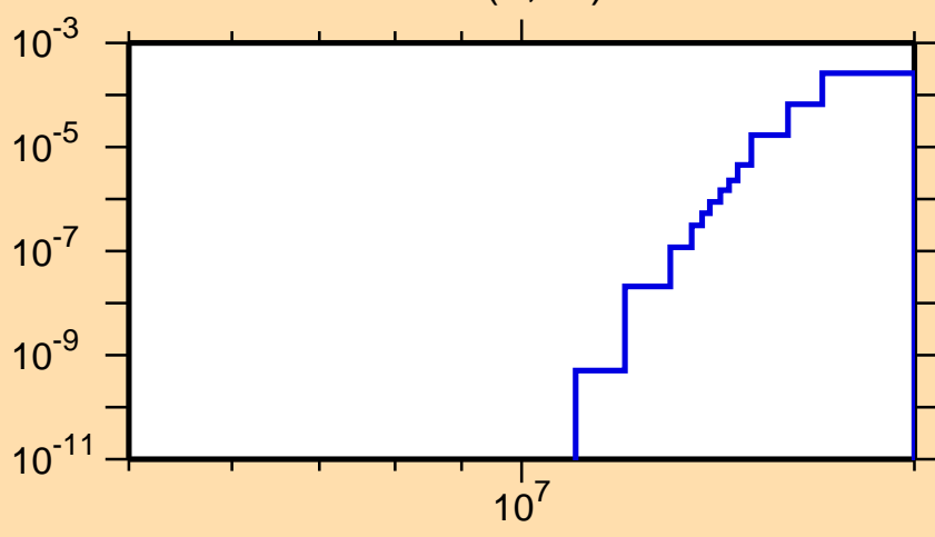
\sigma vs. E for ^{158}\text{Tm}(n,nd)
