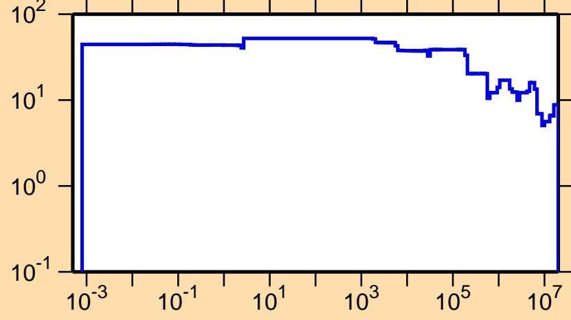
\Delta\sigma/\sigma vs. E for ^{158}\text{Tm}(n,\text{el.})
