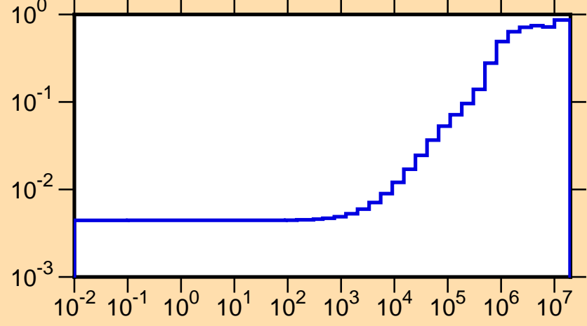
\mu vs. E for ^{158}\text{Tm}(\text{mt251})
