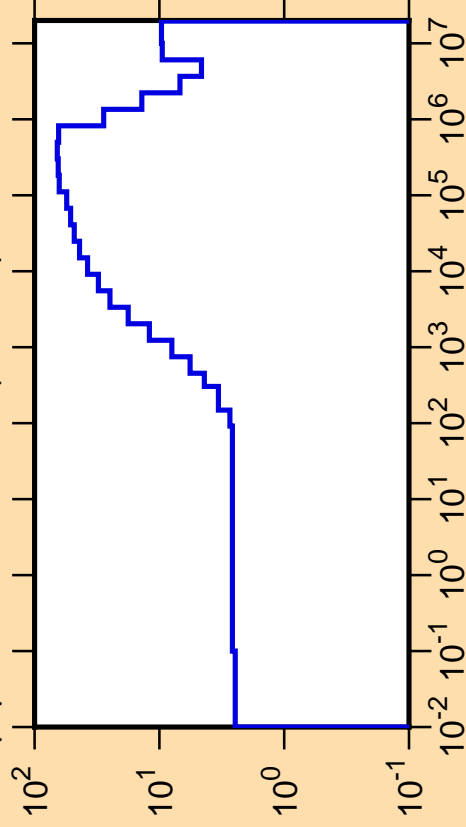
\Delta\mu/\mu vs. E for ^{158}\text{Tm}(\text{mt251})
