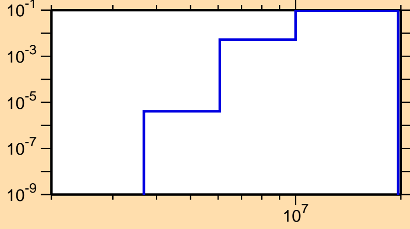
\sigma vs. E for ^{158}\text{Tm}(n,np)
