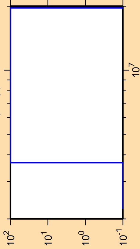
\Delta\sigma/\sigma vs. E for ^{158}\text{Tm}(n,np)
