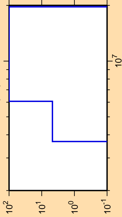
\Delta\sigma/\sigma vs. E for ^{158}\text{Tm}(n,t)
