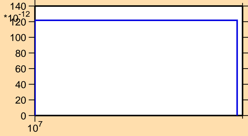
\sigma vs. E for ^{158}\text{Tm}(n,pt)
