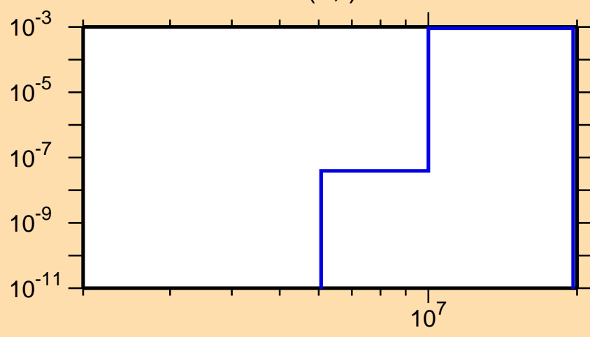
\sigma vs. E for ^{158}\text{Tm}(n,t)
