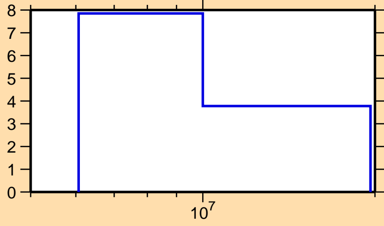
\Delta\sigma/\sigma vs. E for ^{158}\text{Tm}(n,\text{tot.})
