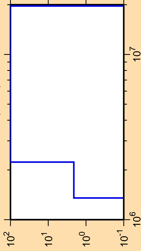
\Delta\sigma/\sigma vs. E for ^{158}\text{Tm}(n,n\alpha)
