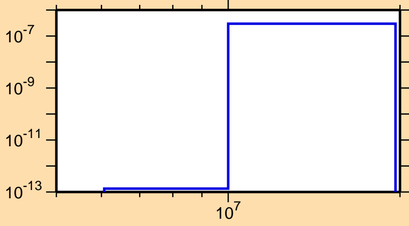
\sigma vs. E for ^{158}\text{Tm} (mt 45)
