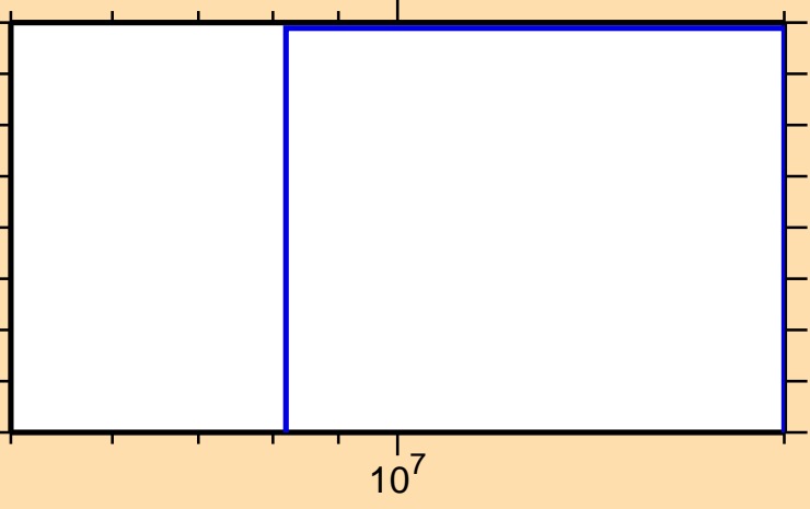
\sigma vs. E for ^{158}\text{Tm}(\text{mt117})
