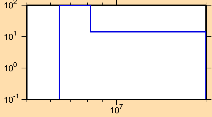
\Delta\sigma/\sigma vs. E for ^{158}\text{Tm}(n,2n)
