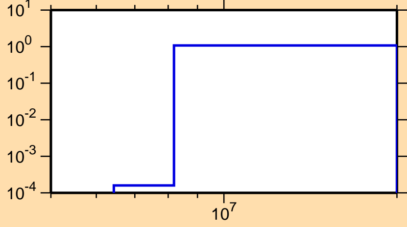
\sigma vs. E for ^{158}\text{Tm}(n,2n)
