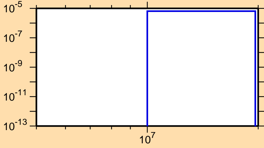
\sigma vs. E for ^{158}\text{Tm}(n,\text{nd})
