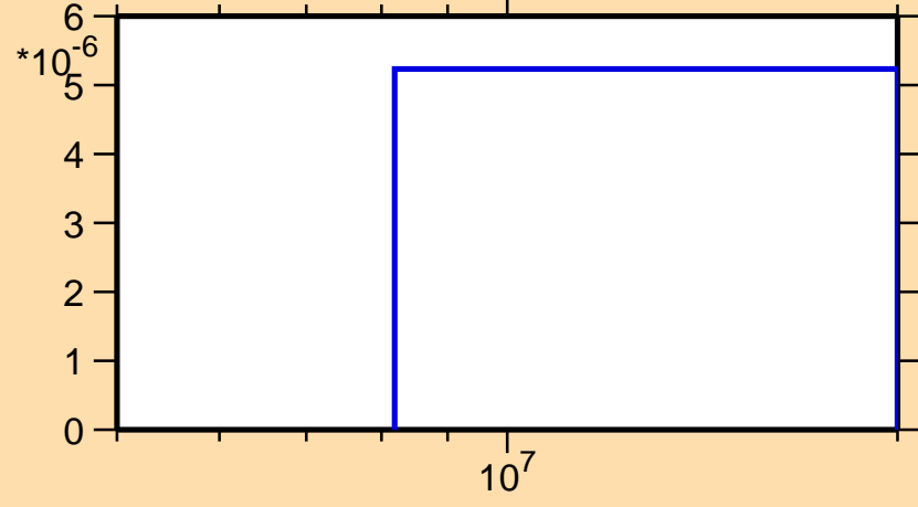
\sigma vs. E for ^{158}\text{Tm}(n,nd)
