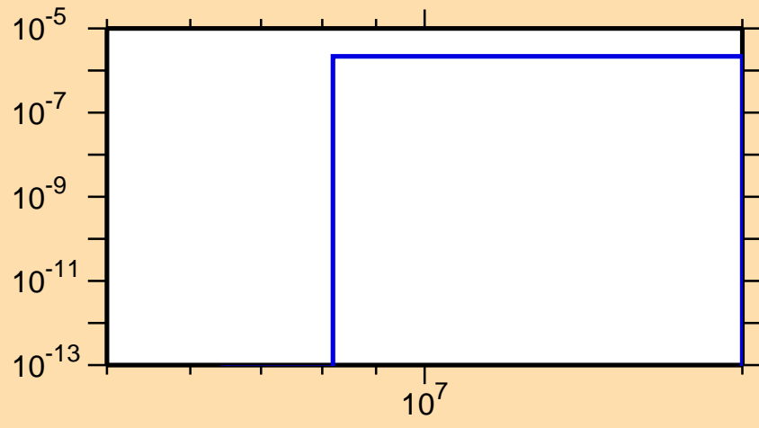
\sigma vs. E for ^{158}\text{Tm}(n,\text{He3})
