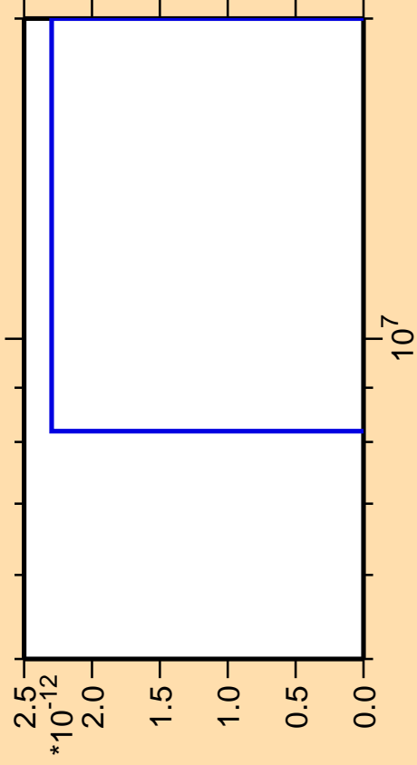
\Delta\sigma/\sigma vs. E for ^{158}\text{Tm} (mt 42)
