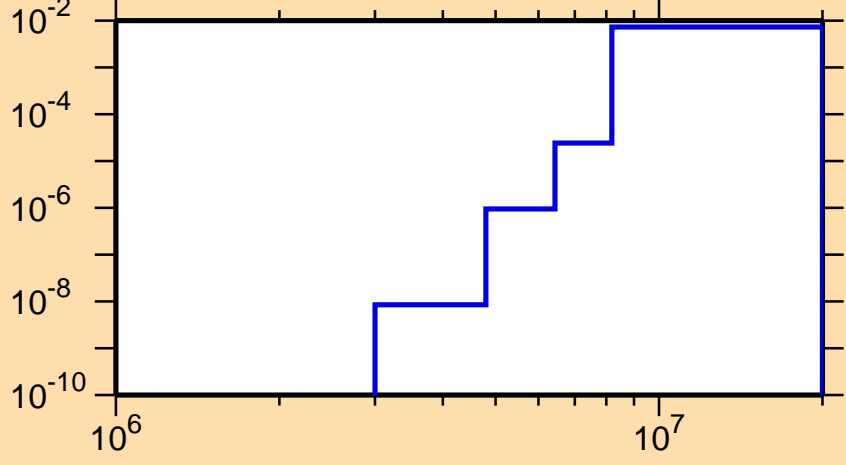
\sigma vs. E for ^{158}\text{Tm}(n,n\alpha)
