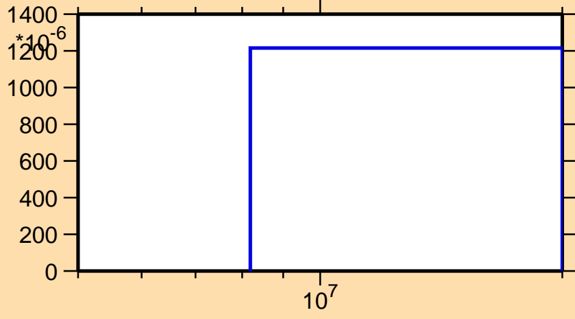
\sigma vs. E for ^{158}\text{Tm}(n,2np)
