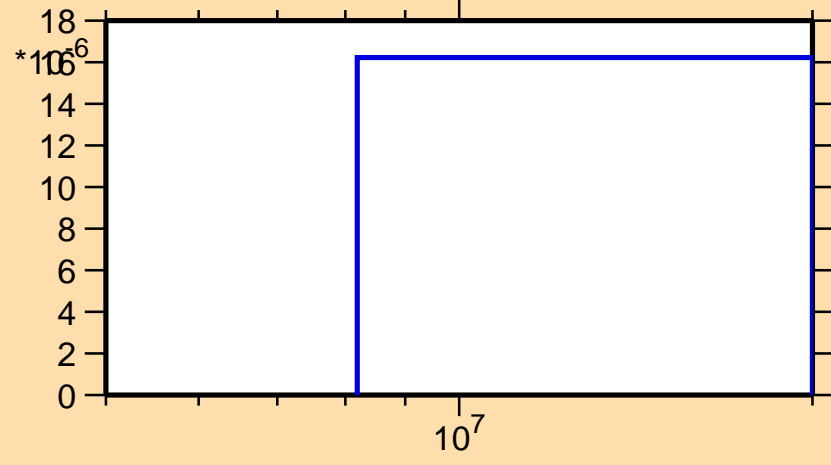
\sigma vs. E for ^{158}\text{Tm}(n,2n\alpha)
