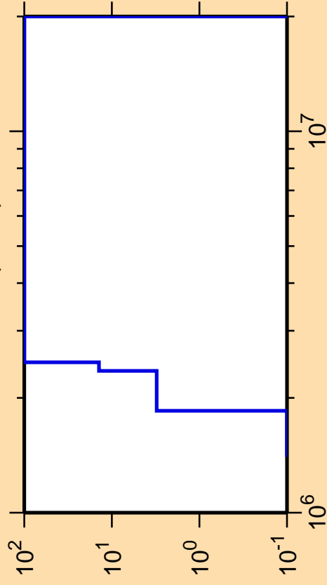
\Delta\sigma/\sigma vs. E for ^{158}\text{Tm}(n,n\alpha)
