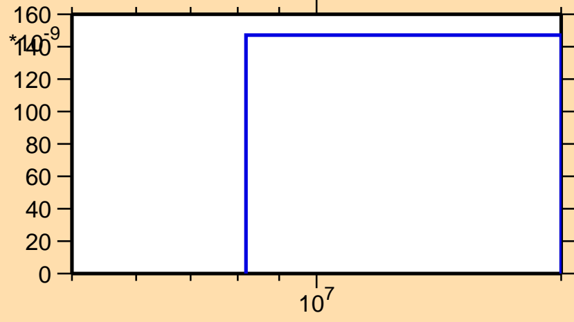
\sigma vs. E for ^{158}\text{Tm} (mt 45)
