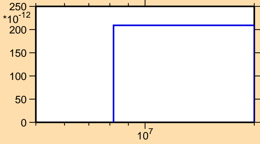
\sigma vs. E for ^{158}\text{Tm}(n,pd)
