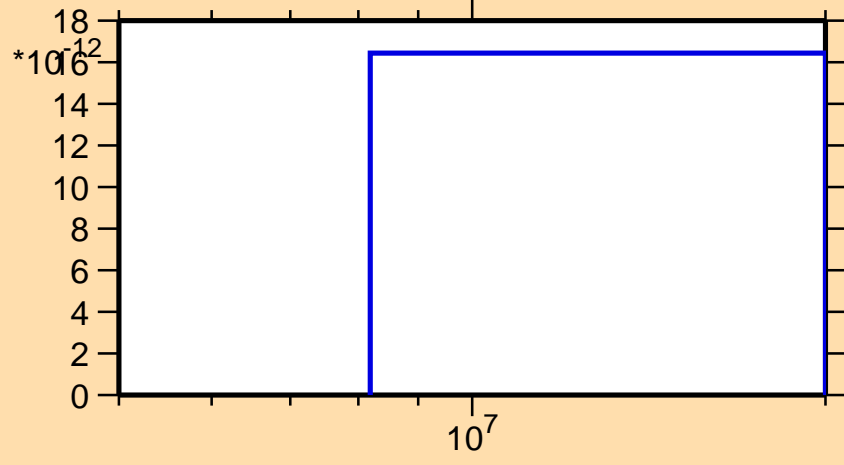
\sigma vs. E for ^{158}\text{Tm} (mt 34)
