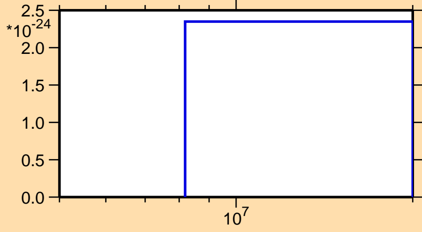
\sigma vs. E for ^{158}\text{Tm} (mt 42)
