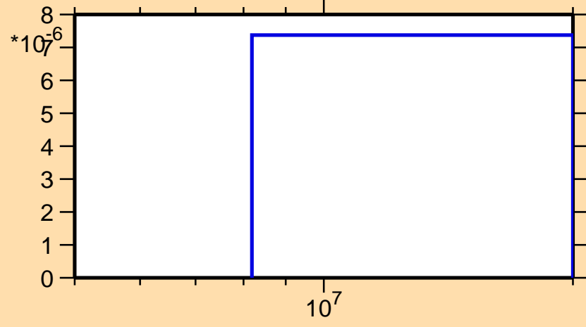
\sigma vs. E for ^{158}\text{Tm}(n,3n)
