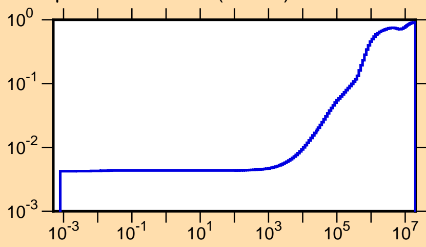
\mu vs. E for ^{159}\text{Tm}(\text{mt251})
