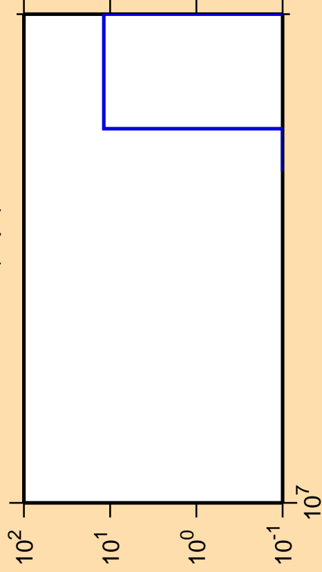
\Delta\sigma/\sigma vs. E for ^{159}\text{Tm}(n,pt)
