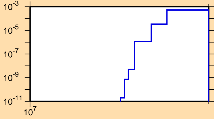
\sigma vs. E for ^{159}\text{Tm}(n,2np)
