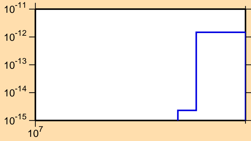
\sigma vs. E for ^{159}\text{Tm}(n,pt)
