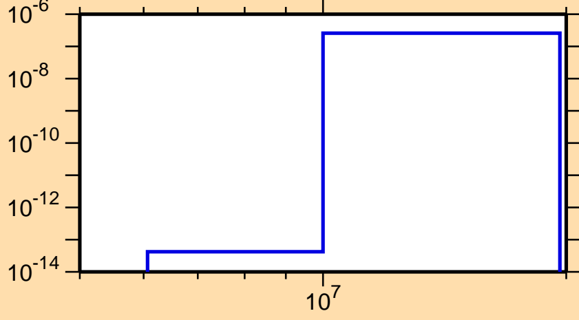
\sigma vs. E for ^{159}\text{Tm}(n,\text{He3})
