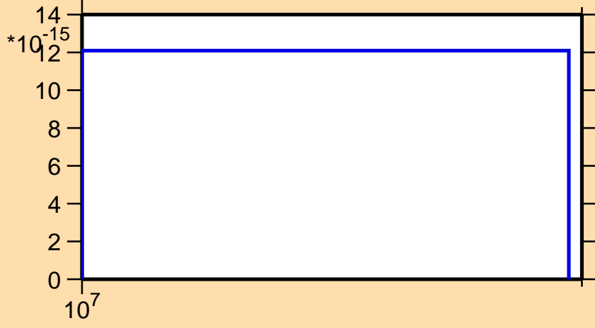
\sigma vs. E for ^{159}\text{Tm} (mt 34)
