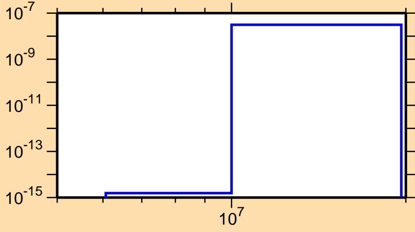
\sigma vs. E for ^{159}\text{Tm} (mt 45)
