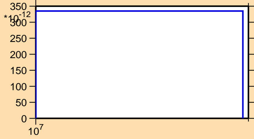
\sigma vs. E for ^{159}\text{Tm}(n,pd)
