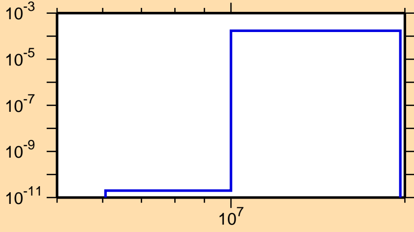
\sigma vs. E for ^{159}\text{Tm}(n,t)
