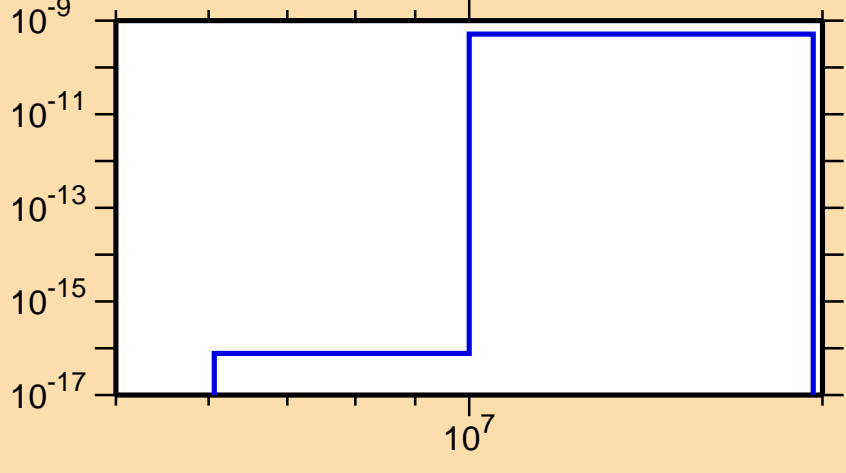
\sigma vs. E for ^{159}\text{Tm}(\text{mt117})
