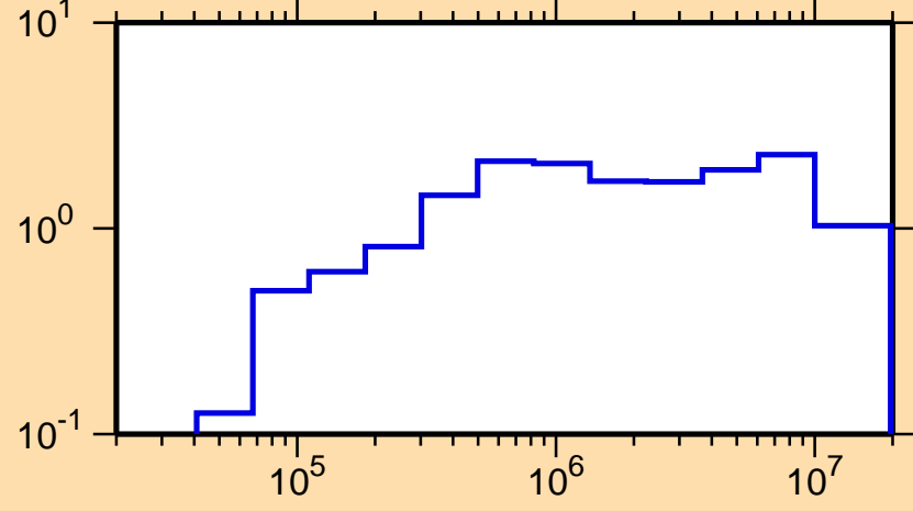
\sigma vs. E for ^{159}\text{Tm}(n,\text{inel.})
