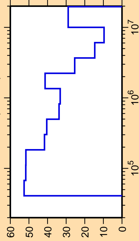
\Delta\sigma/\sigma vs. E for ^{159}\text{Tm}(n,\text{inel.})
