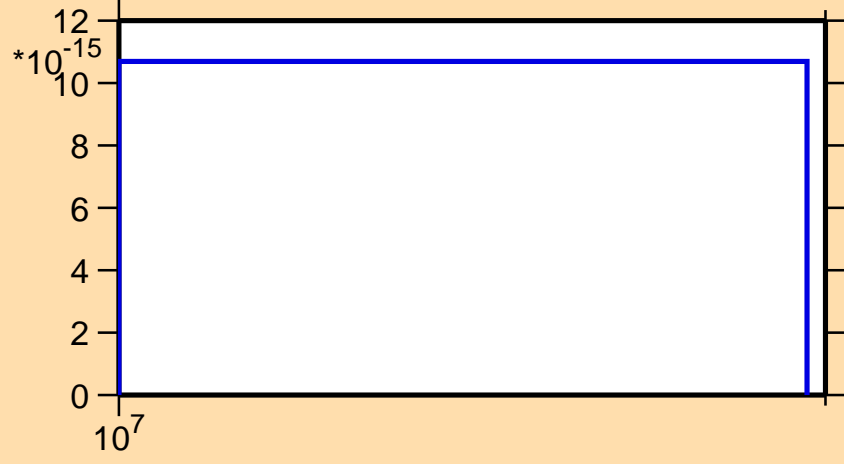
\sigma vs. E for ^{159}\text{Tm}(n,pt)
