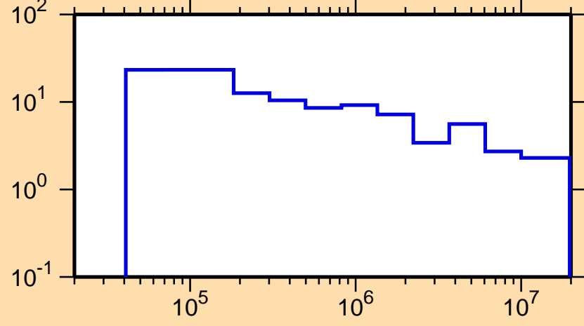
\Delta\sigma/\sigma vs. E for ^{159}\text{Tm}(n,\text{tot.})
