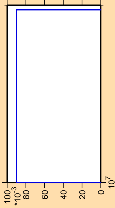
\Delta\sigma/\sigma vs. E for ^{159}\text{Tm} (mt 34)
