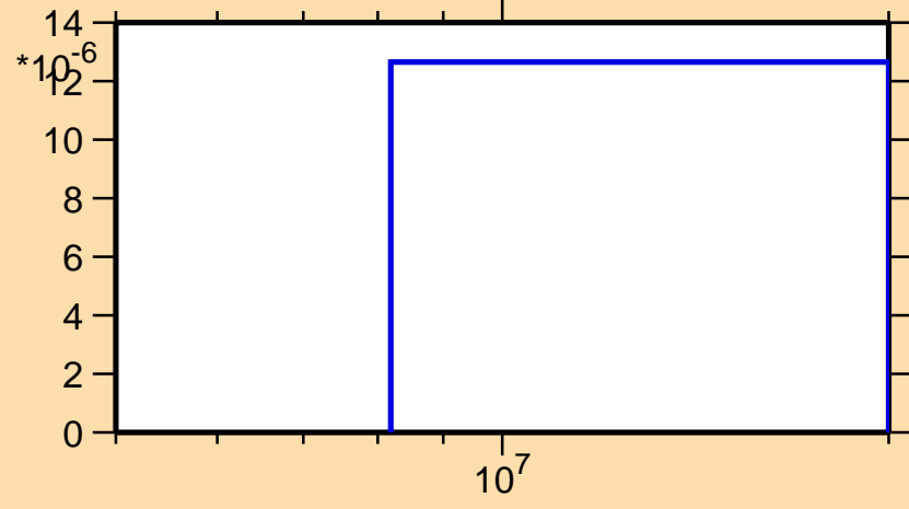
\sigma vs. E for ^{159}\text{Tm}(n,3n)
