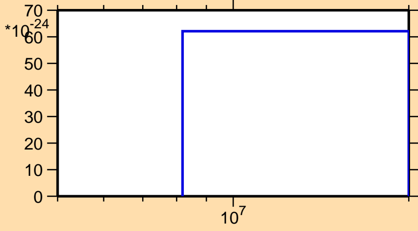
\sigma vs. E for ^{159}\text{Tm} (mt 42)
