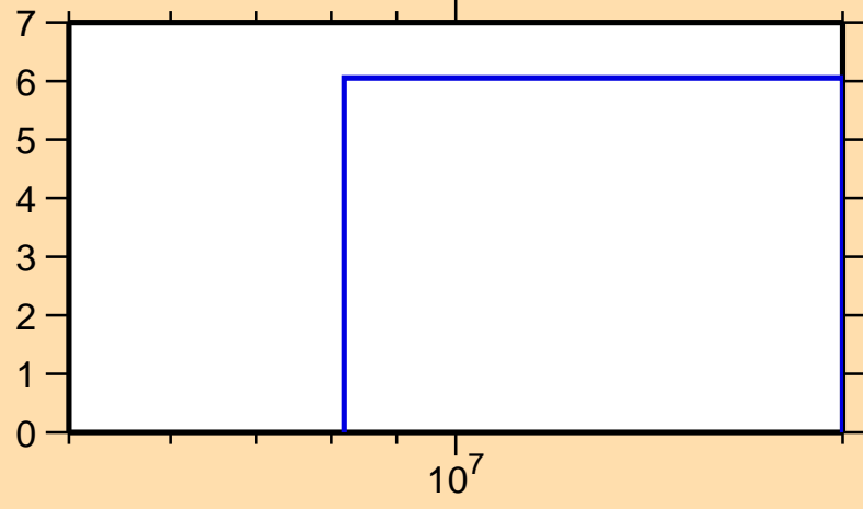
\Delta\sigma/\sigma vs. E for ^{159}\text{Tm}(n,el.)
