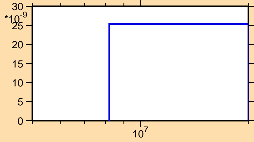
\sigma vs. E for ^{159}\text{Tm} (mt 45)
