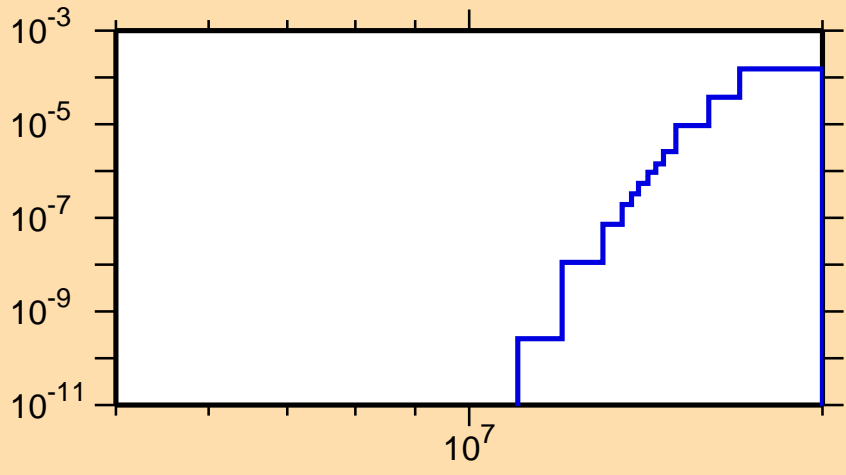
\sigma vs. E for ^{160}\text{Tm}(n,2n\alpha)
