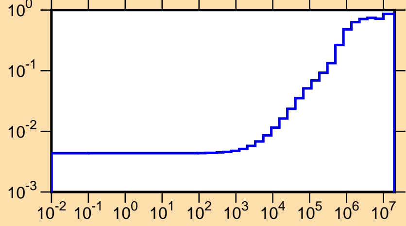
\mu vs. E for ^{160}\text{Tm}(\text{mt251})
