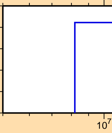
\sigma vs. E for ^{160}\text{Tm}(n,2n\alpha)
