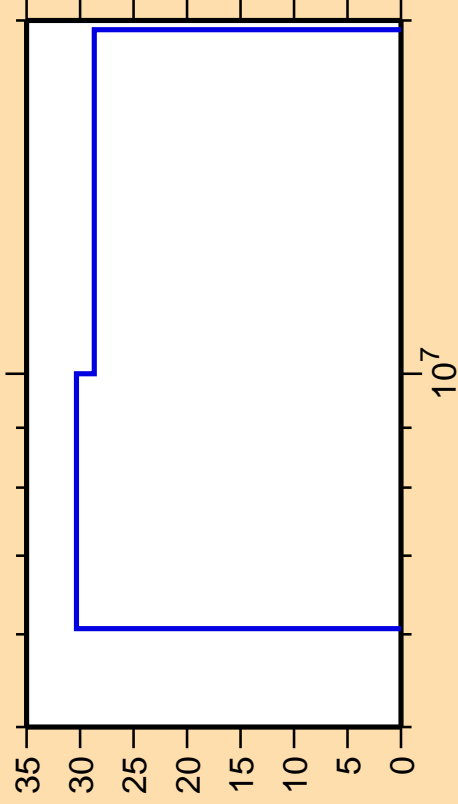
\Delta\sigma/\sigma vs. E for ^{160}\text{Tm}(n,p)
