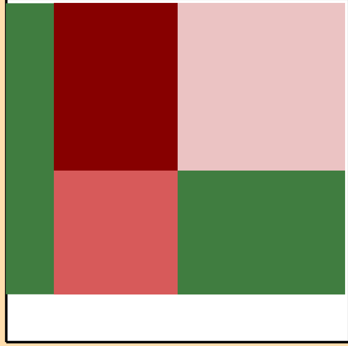
\Delta\sigma/\sigma vs. E for ^{160}\text{Tm}(n,\text{el.})
