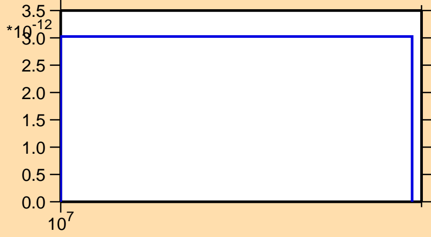
\sigma vs. E for ^{160}\text{Tm}(n,pt)
