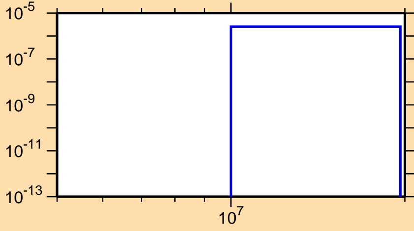
\sigma vs. E for ^{160}\text{Tm}(n,nd)
