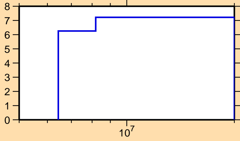
\Delta\sigma/\sigma vs. E for ^{160}\text{Tm}(n,\text{tot.})
