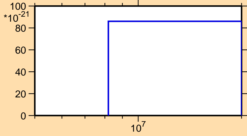
\sigma vs. E for ^{160}\text{Tm} (mt 11)
