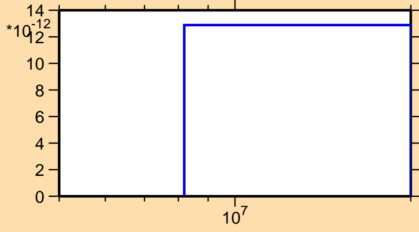
\sigma vs. E for ^{160}\text{Tm}(n,pd)
