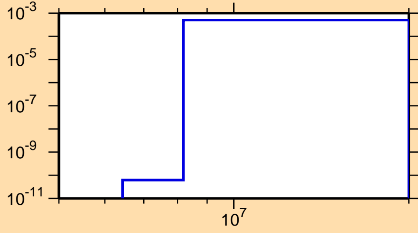
\sigma vs. E for ^{160}\text{Tm}(n,t)
