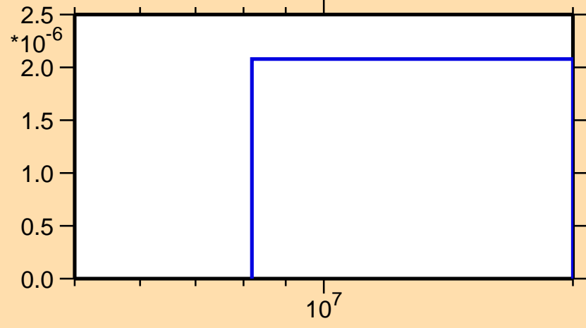
\sigma vs. E for ^{160}\text{Tm}(n,nd)
