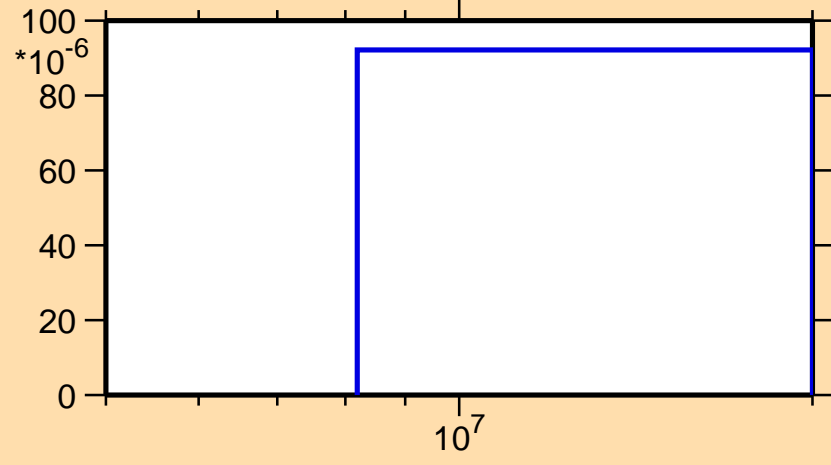
\sigma vs. E for ^{160}\text{Tm}(n,2np)
