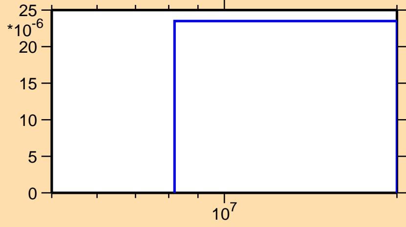
\sigma vs. E for ^{160}\text{Tm}(n,3n)
