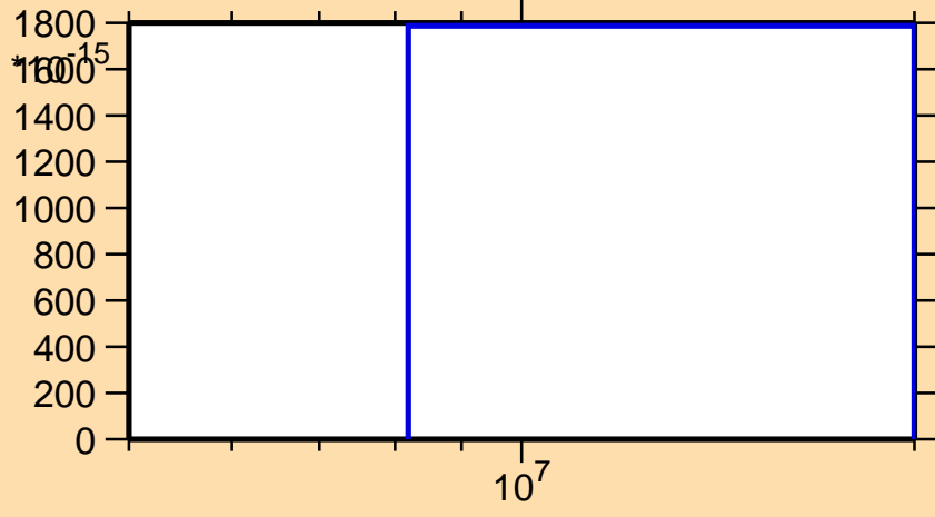
\sigma vs. E for ^{160}\text{Tm} (mt 34)
