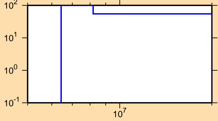
\Delta\sigma/\sigma vs. E for ^{160}\text{Tm}(n,2n)
