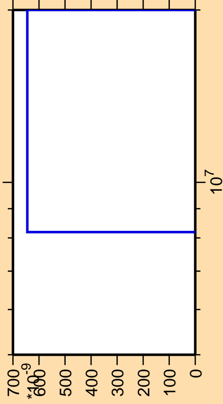
\Delta\sigma/\sigma vs. E for ^{160}\text{Tm} (mt 11)
