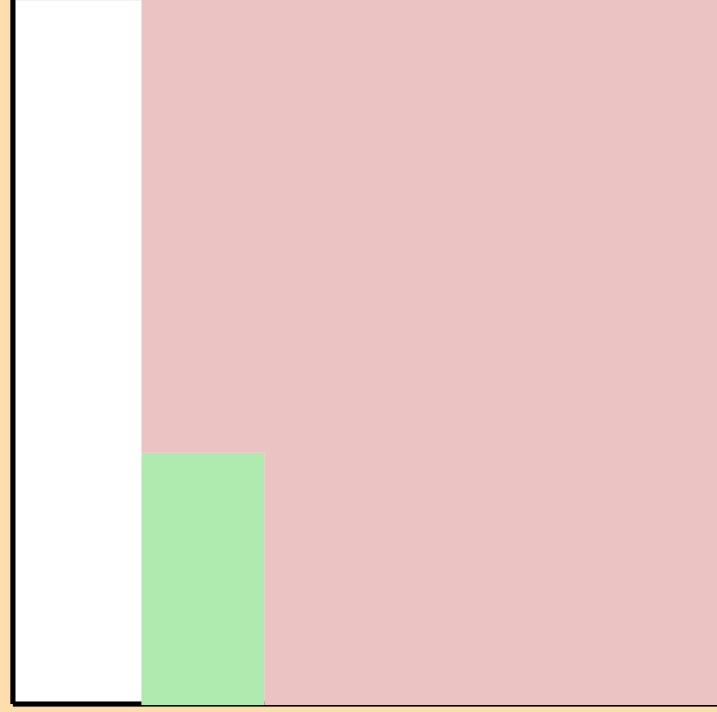
\Delta\sigma/\sigma vs. E for ^{160}\text{Tm}(n,2n)
