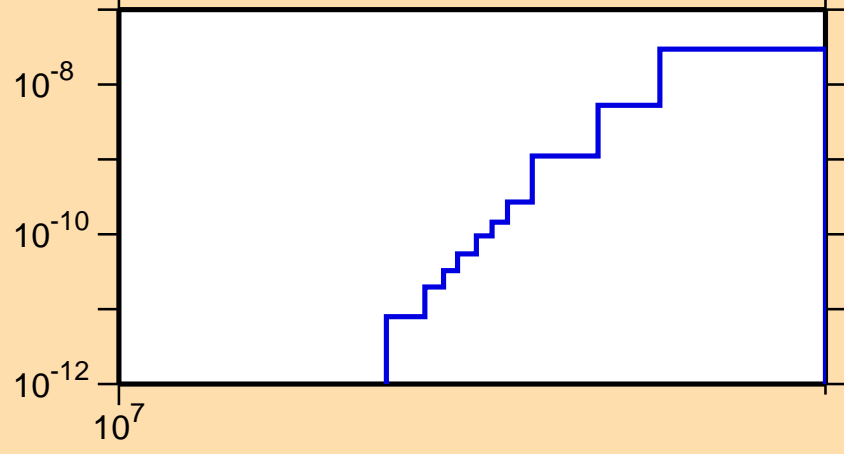
\sigma vs. E for ^{161}\text{Tm} (mt 45)
