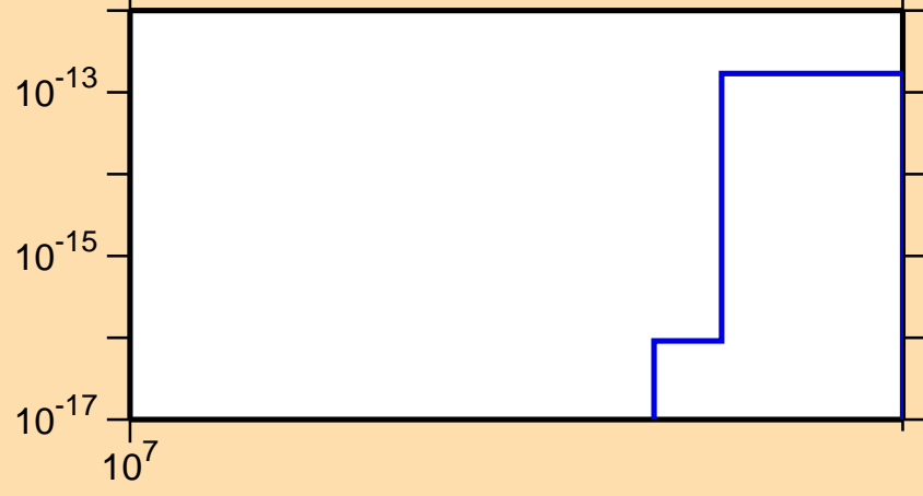
\sigma vs. E for ^{161}\text{Tm}(n,pt)
