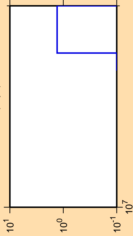
\Delta\sigma/\sigma vs. E for ^{161}\text{Tm}(n,pt)
