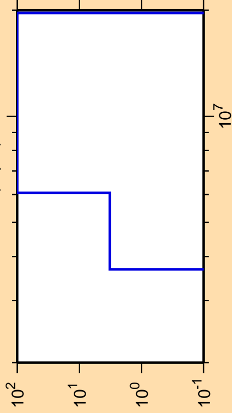
\Delta\sigma/\sigma vs. E for ^{161}\text{Tm}(n,p\alpha)
