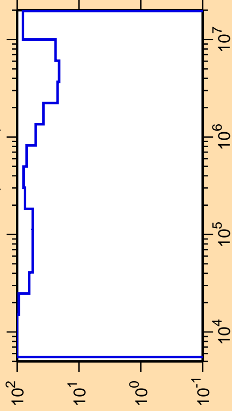
\Delta\sigma/\sigma vs. E for ^{161}\text{Tm}(n,\text{inel.})
