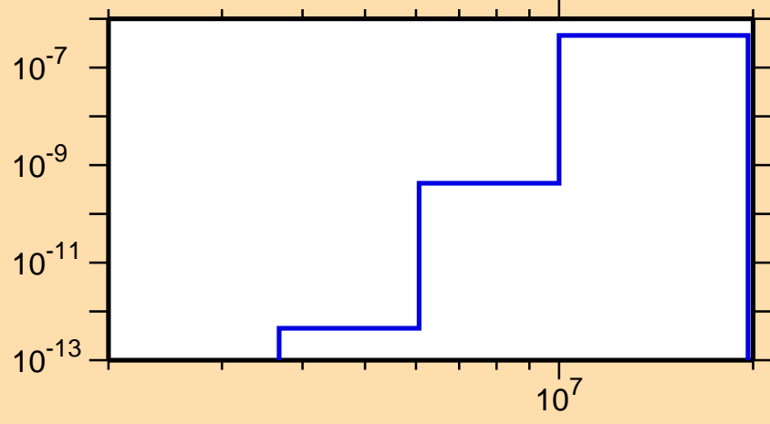
\sigma vs. E for ^{161}\text{Tm}(n,p\alpha)
