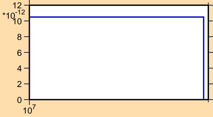
\sigma vs. E for ^{161}\text{Tm}(n,pd)
