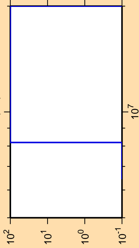
\Delta\sigma/\sigma vs. E for ^{161}\text{Tm}(n,t)
