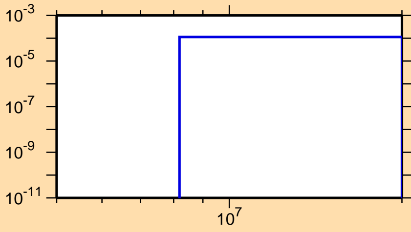
\sigma vs. E for ^{161}\text{Tm}(n,t)
