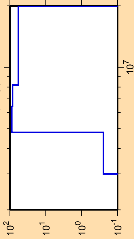
\Delta\sigma/\sigma vs. E for ^{161}\text{Tm}(n,np)
