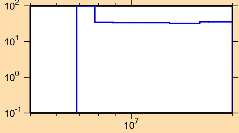
\Delta\sigma/\sigma vs. E for ^{162}\text{Tm}(n,2n)
