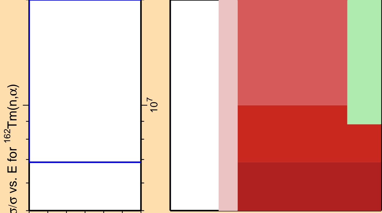
\Delta\sigma/\sigma vs. E for ^{162}\text{Tm}(n,2n)
