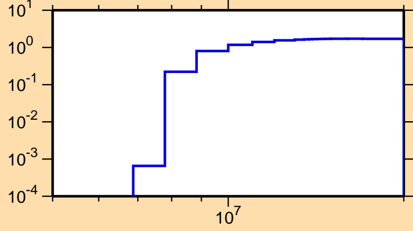
\sigma vs. E for ^{162}\text{Tm}(n,2n)
