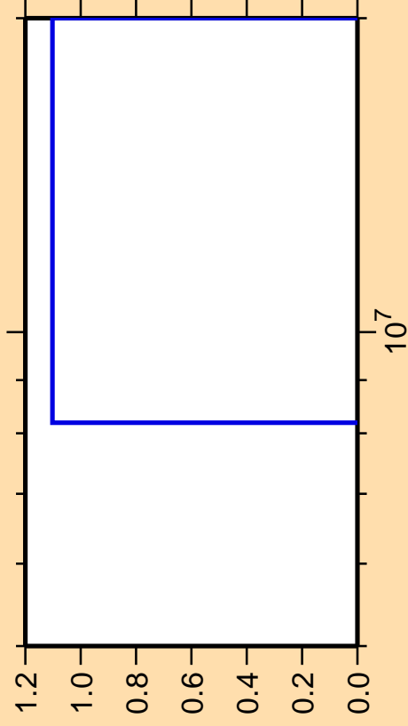
\Delta\sigma/\sigma vs. E for ^{162}\text{Tm}(n,pt)
