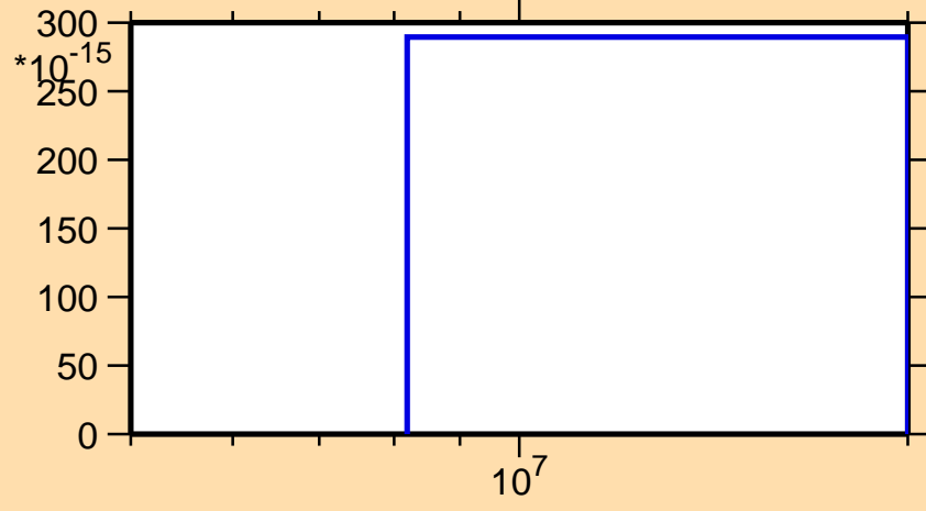
\sigma vs. E for ^{162}\text{Tm}(n,pt)
