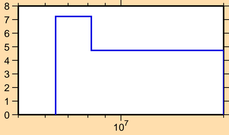
\Delta\sigma/\sigma vs. E for ^{162}\text{Tm}(n,\text{tot.})
