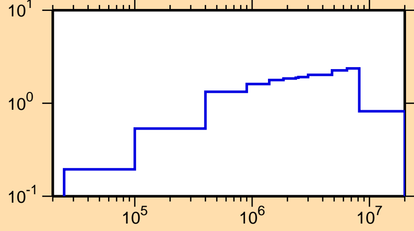
\sigma vs. E for ^{162}\text{Tm}(n,\text{inel.})
