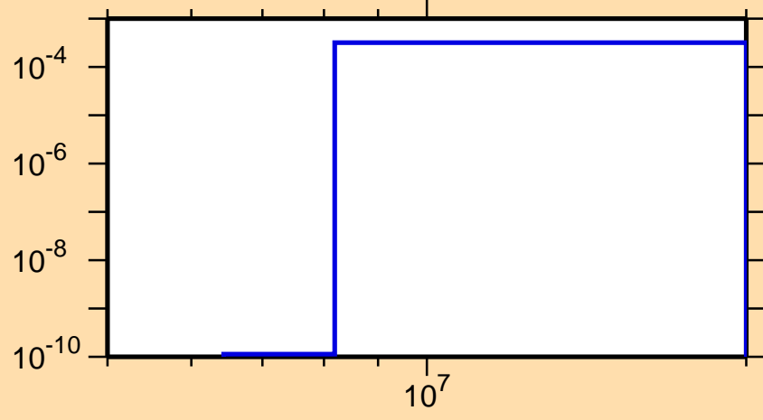
\sigma vs. E for ^{162}\text{Tm}(n,t)
