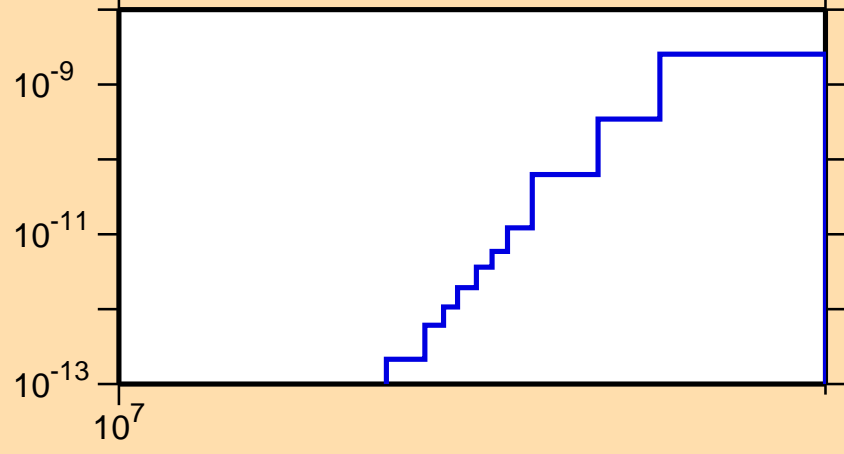
\sigma vs. E for ^{162}\text{Tm} (mt 45)
