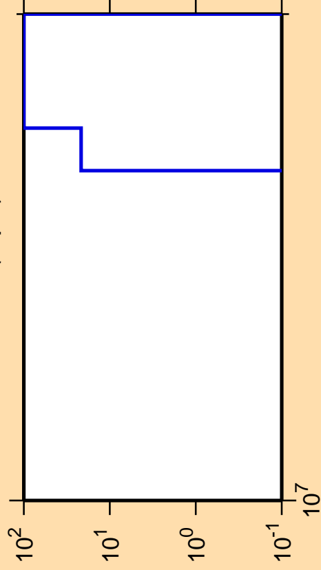
\Delta\sigma/\sigma vs. E for ^{162}\text{Tm}(n,pd)
