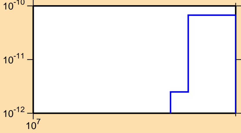
\sigma vs. E for ^{162}\text{Tm}(n,pd)
