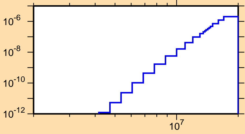
\sigma vs. E for ^{162}\text{Tm}(n,p\alpha)
