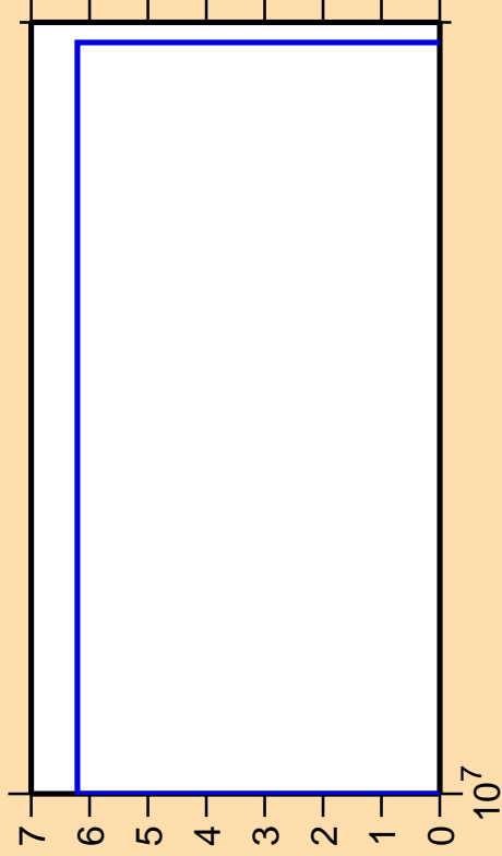
\Delta\sigma/\sigma vs. E for ^{162}\text{Tm}(n,pd)
