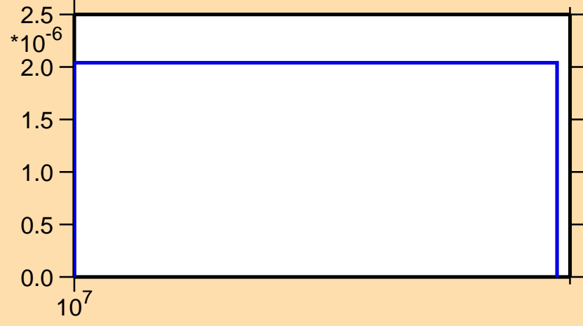
\sigma vs. E for ^{162}\text{Tm}(n,nd)
